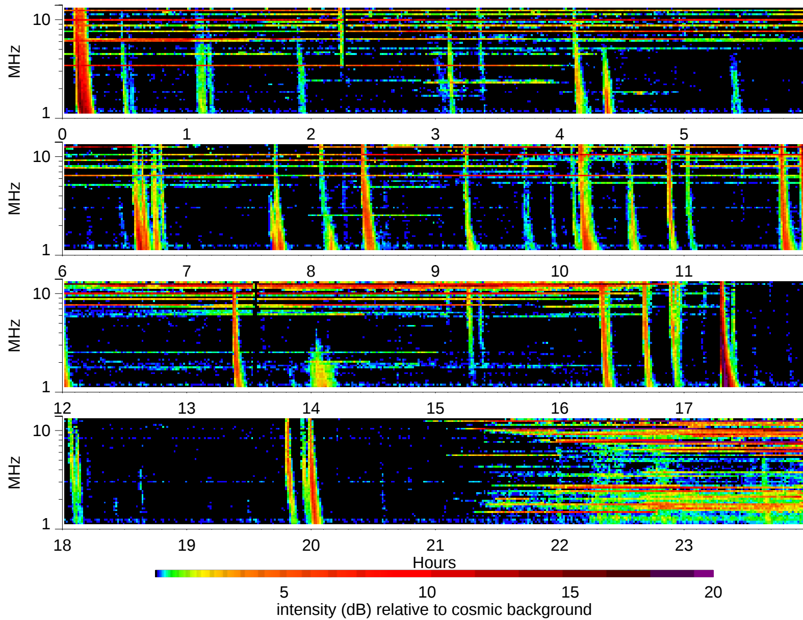
Wind Waves RAD2 receiver: 1999/3/11
