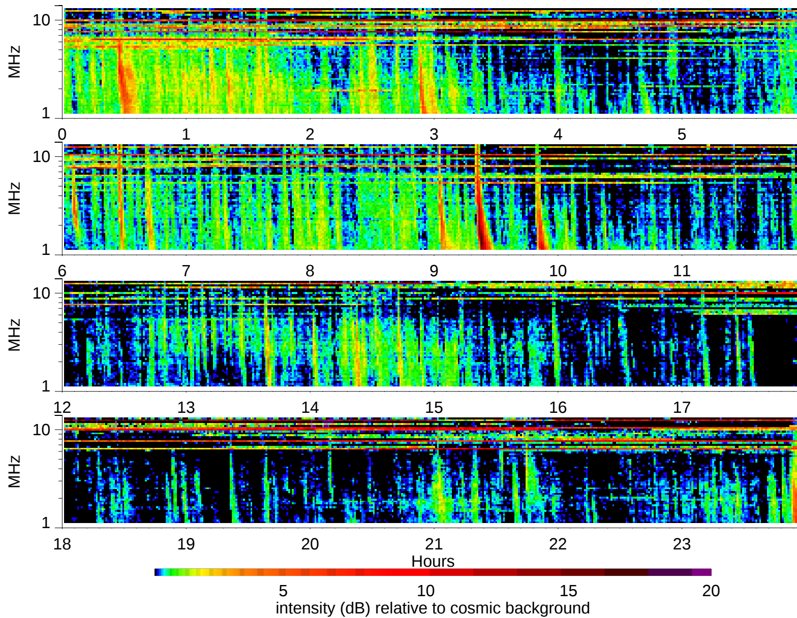
Wind Waves RAD2 receiver: 1999/3/14
