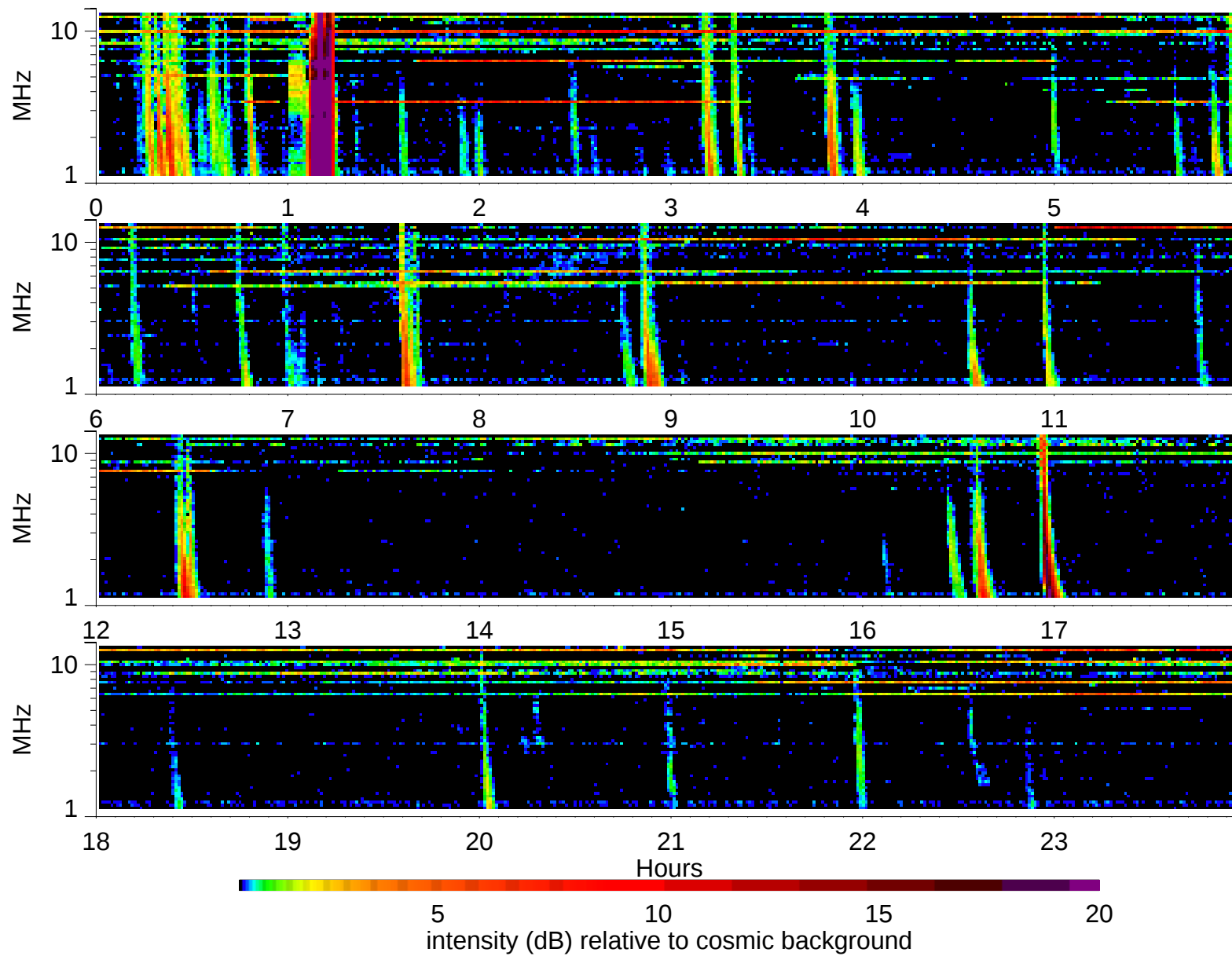
Wind Waves RAD2 receiver: 1999/3/21
