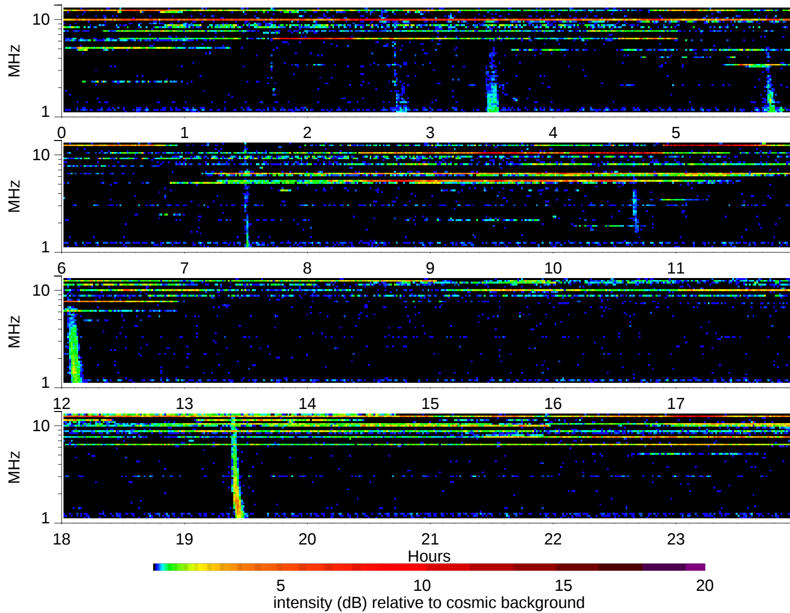
Wind Waves RAD2 receiver: 1999/3/22
