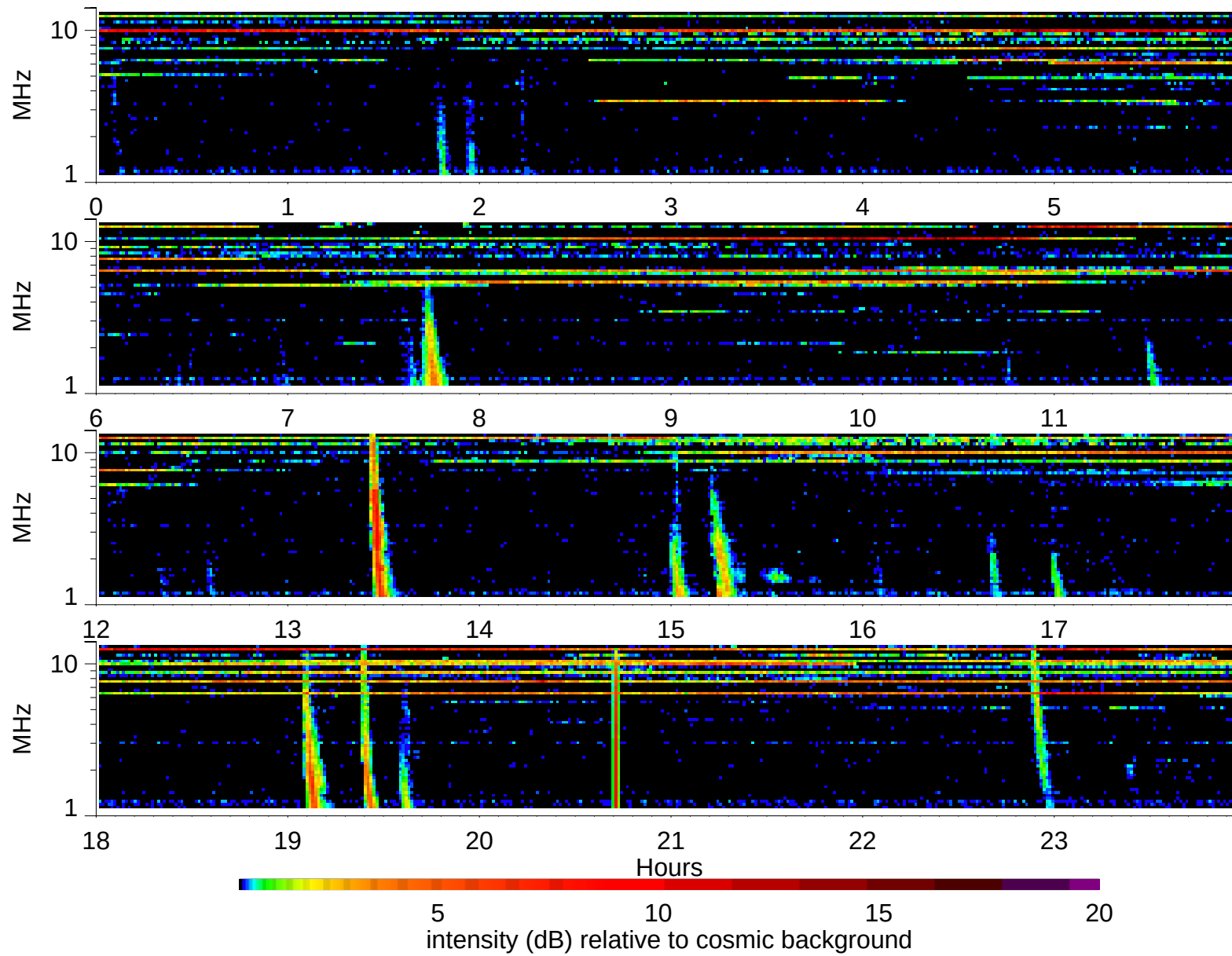
Wind Waves RAD2 receiver: 1999/3/24
