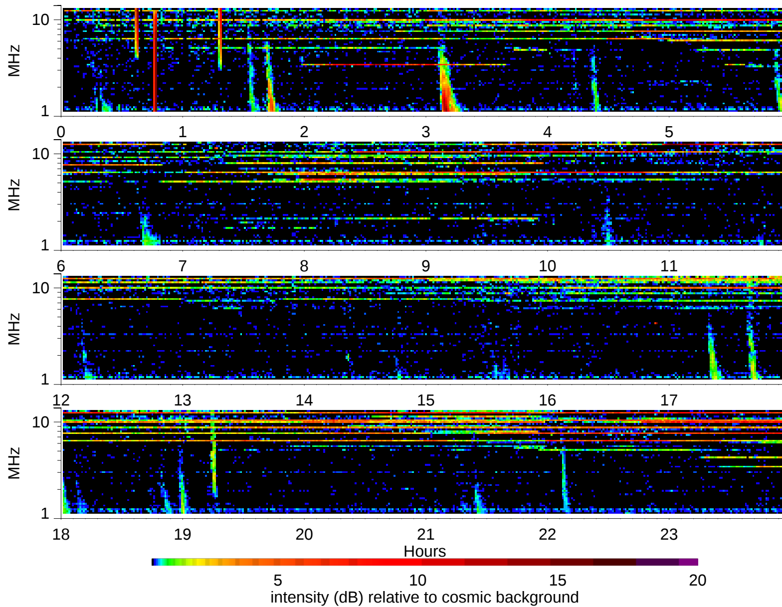
Wind Waves RAD2 receiver: 1999/3/26
