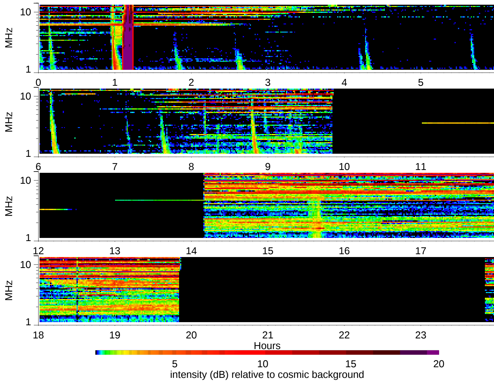
Wind Waves RAD2 receiver: 1999/3/29
