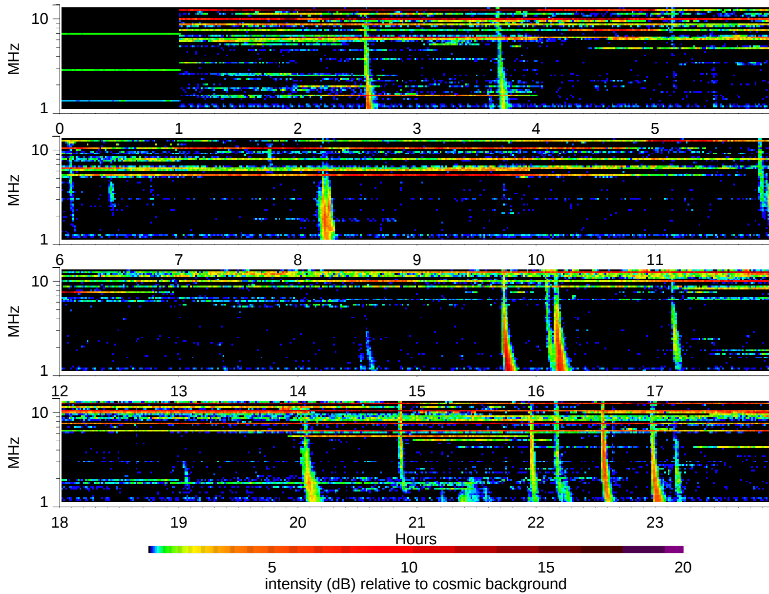
Wind Waves RAD2 receiver: 1999/4/2
