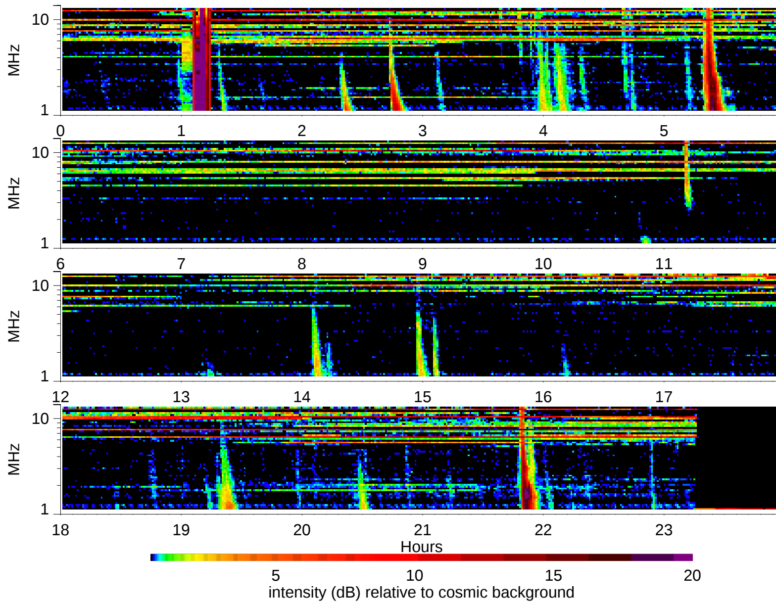
Wind Waves RAD2 receiver: 1999/4/4
