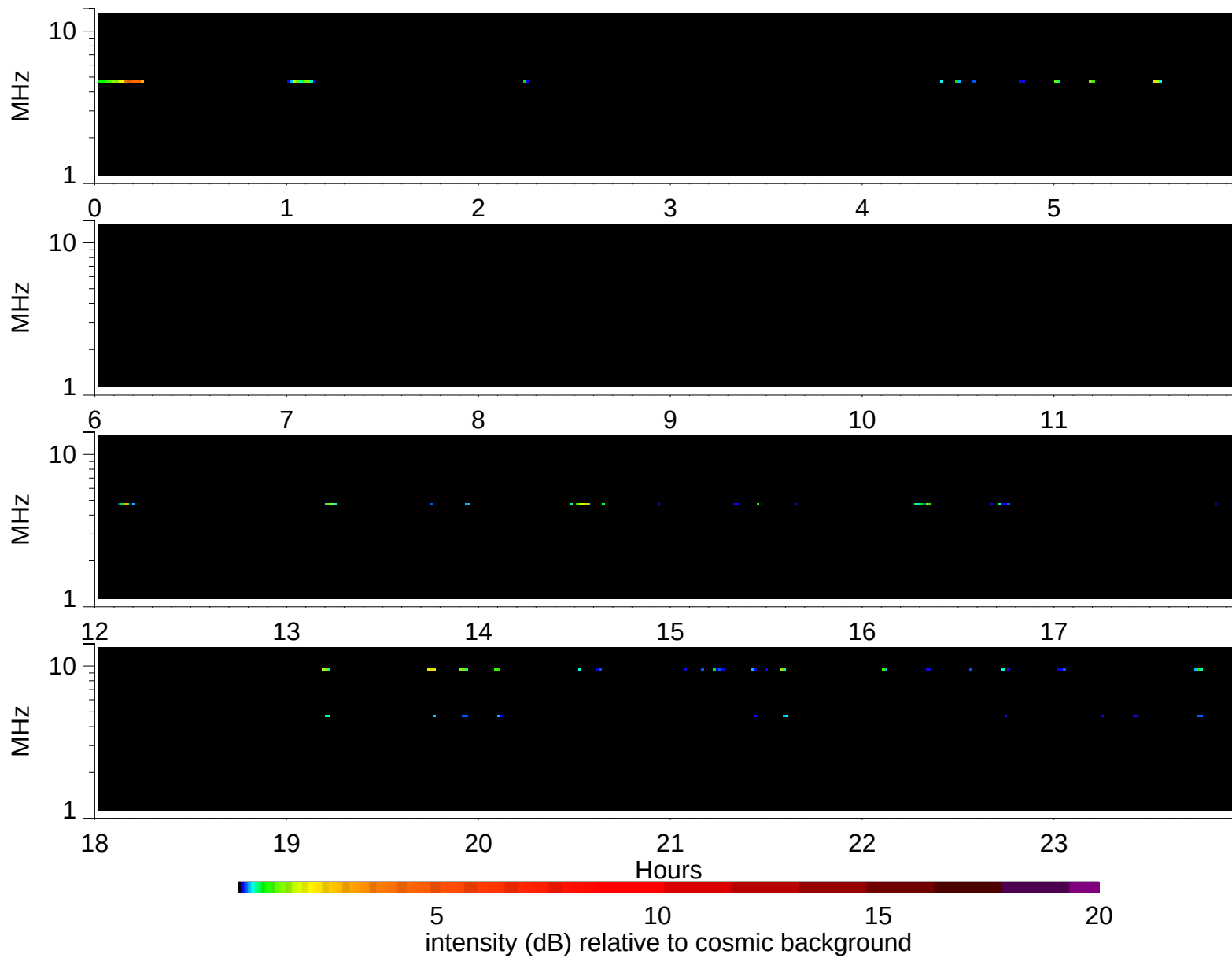
Wind Waves RAD2 receiver: 1999/4/5
