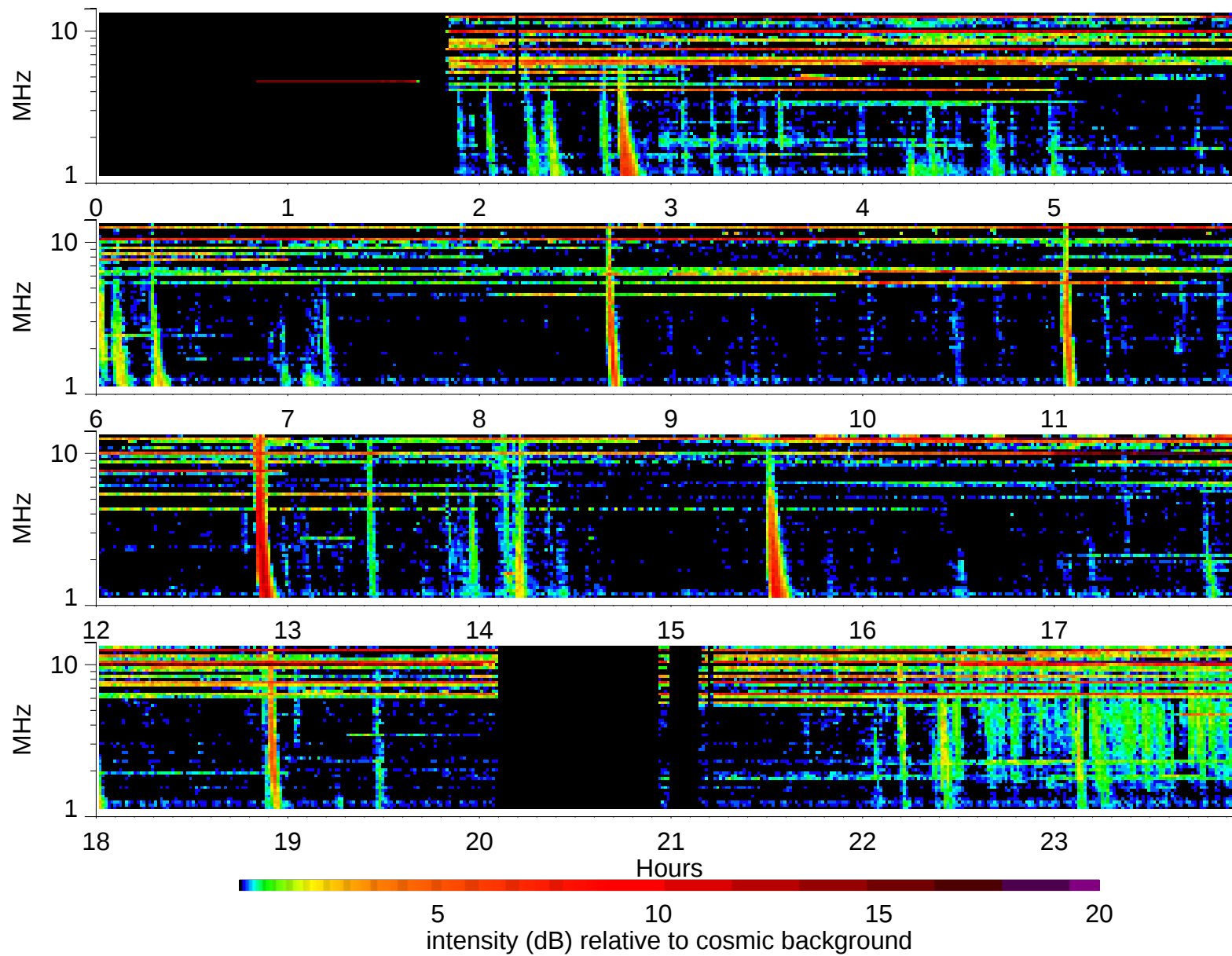
Wind Waves RAD2 receiver: 1999/4/7
