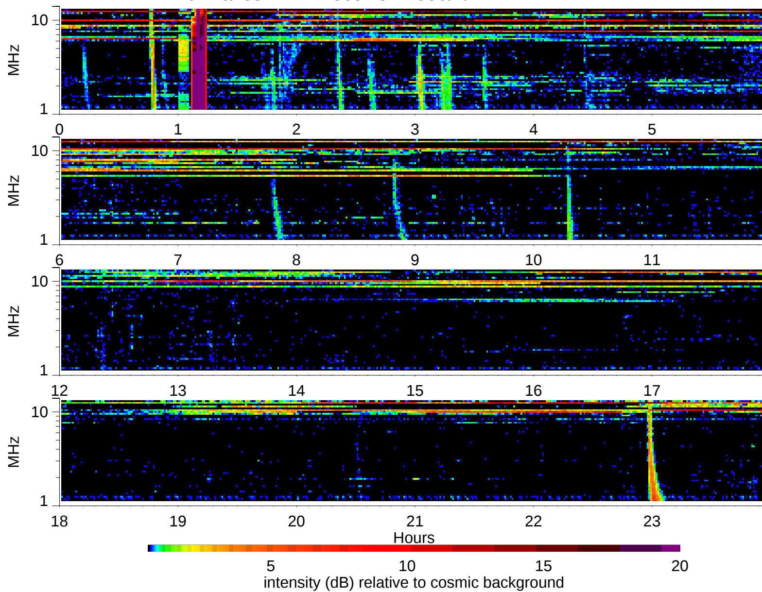
Wind Waves RAD2 receiver: 1999/4/12
