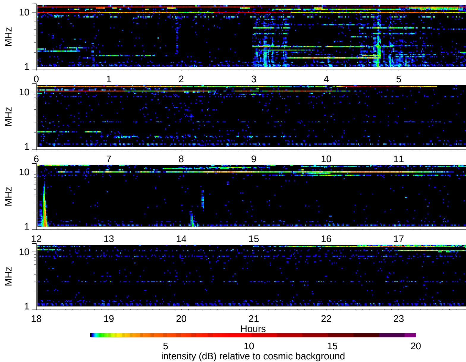
Wind Waves RAD2 receiver: 1999/4/13
