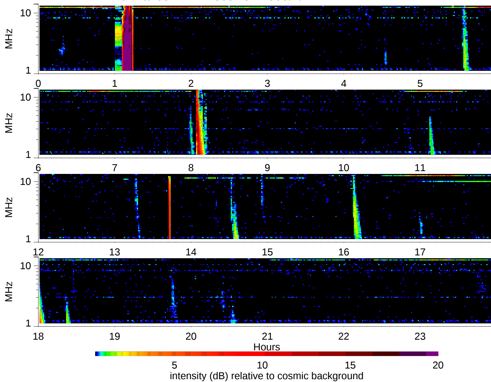
Wind Waves RAD2 receiver: 1999/4/14
