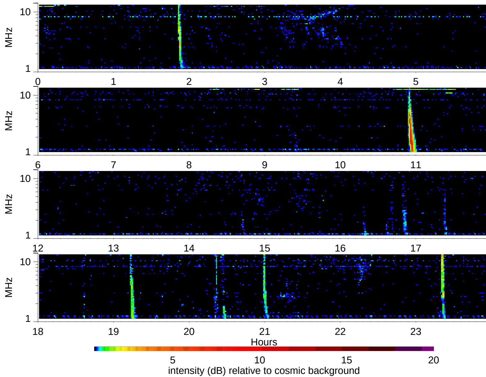
Wind Waves RAD2 receiver: 1999/4/15
