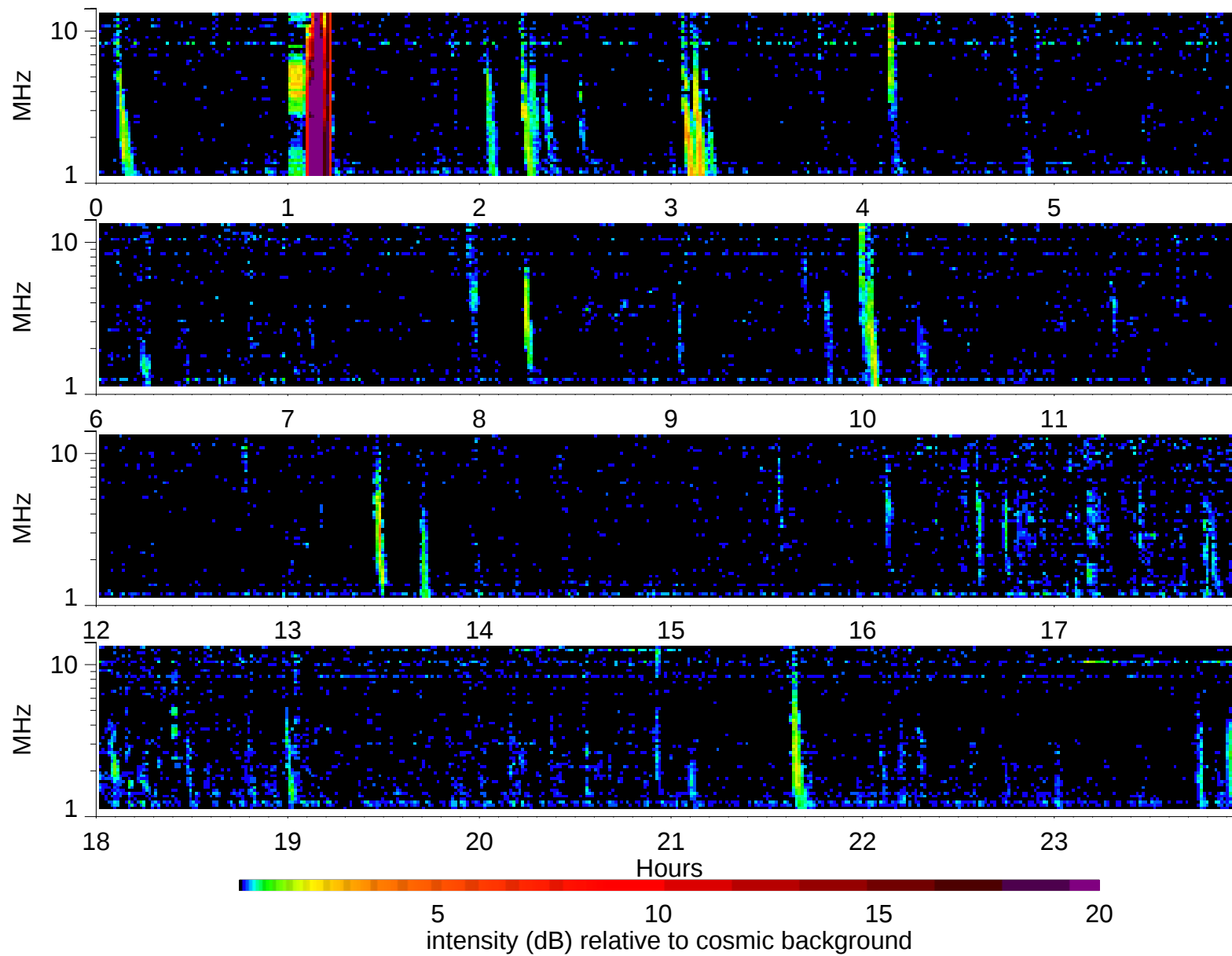
Wind Waves RAD2 receiver: 1999/4/16
