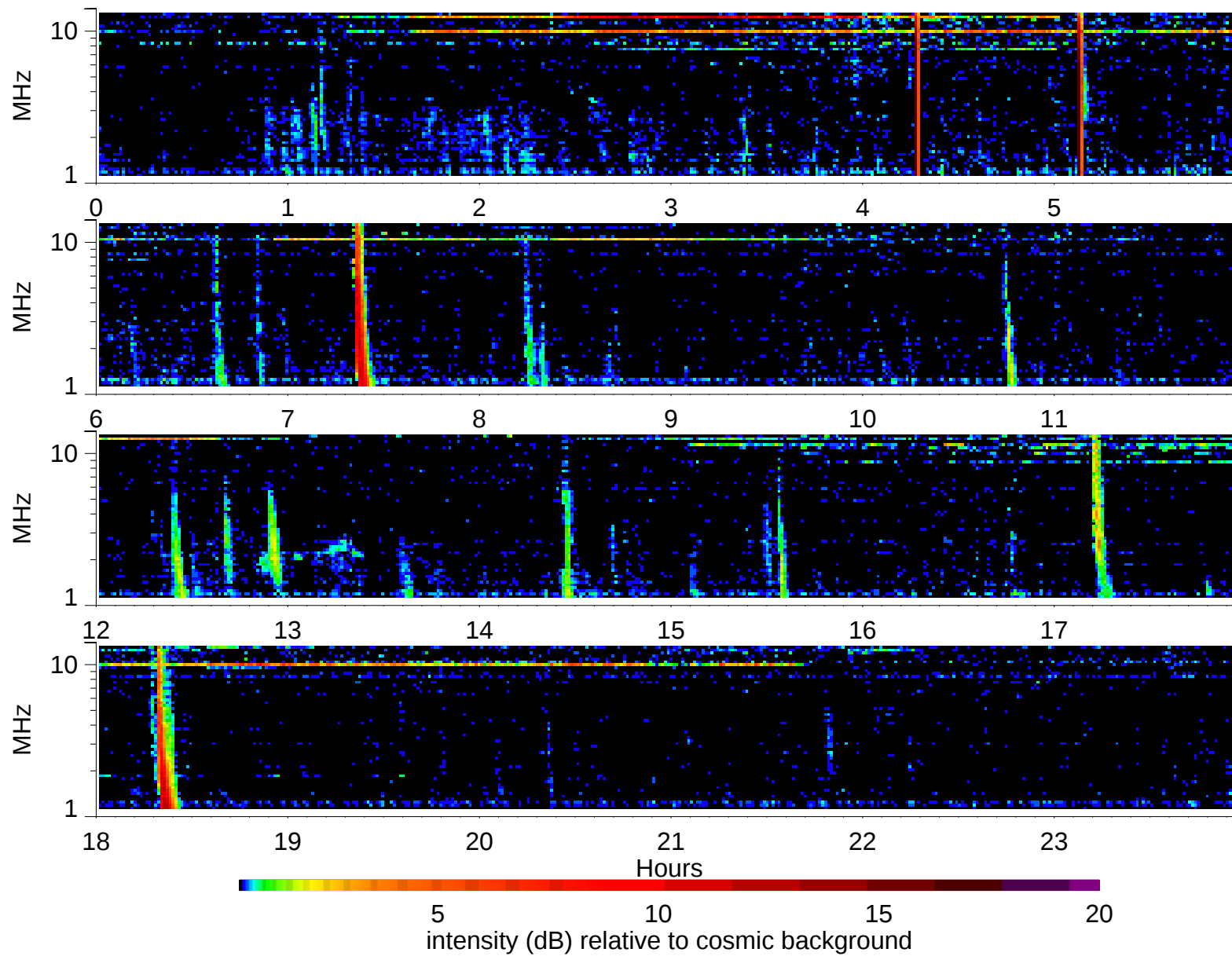
Wind Waves RAD2 receiver: 1999/4/17
