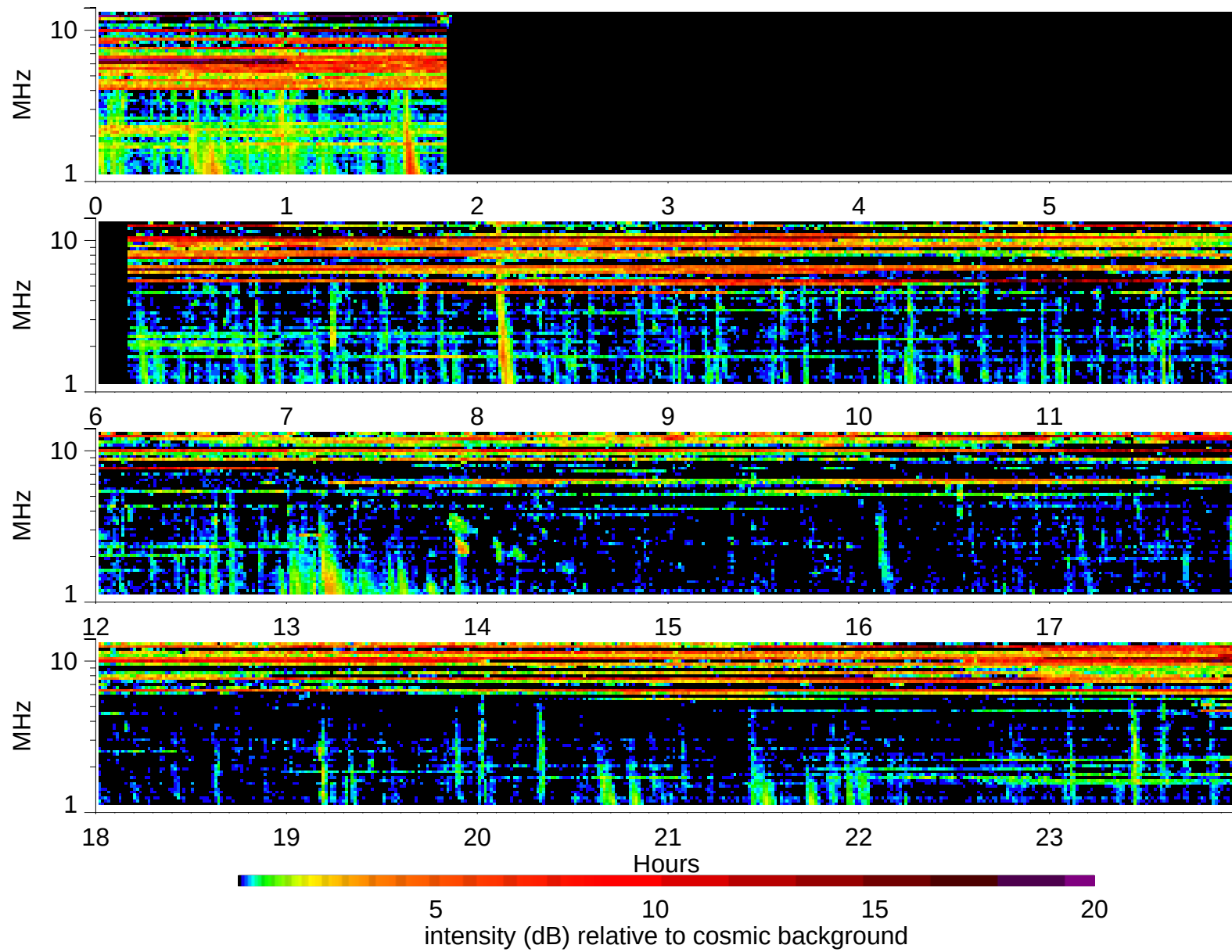
Wind Waves RAD2 receiver: 1999/4/24
