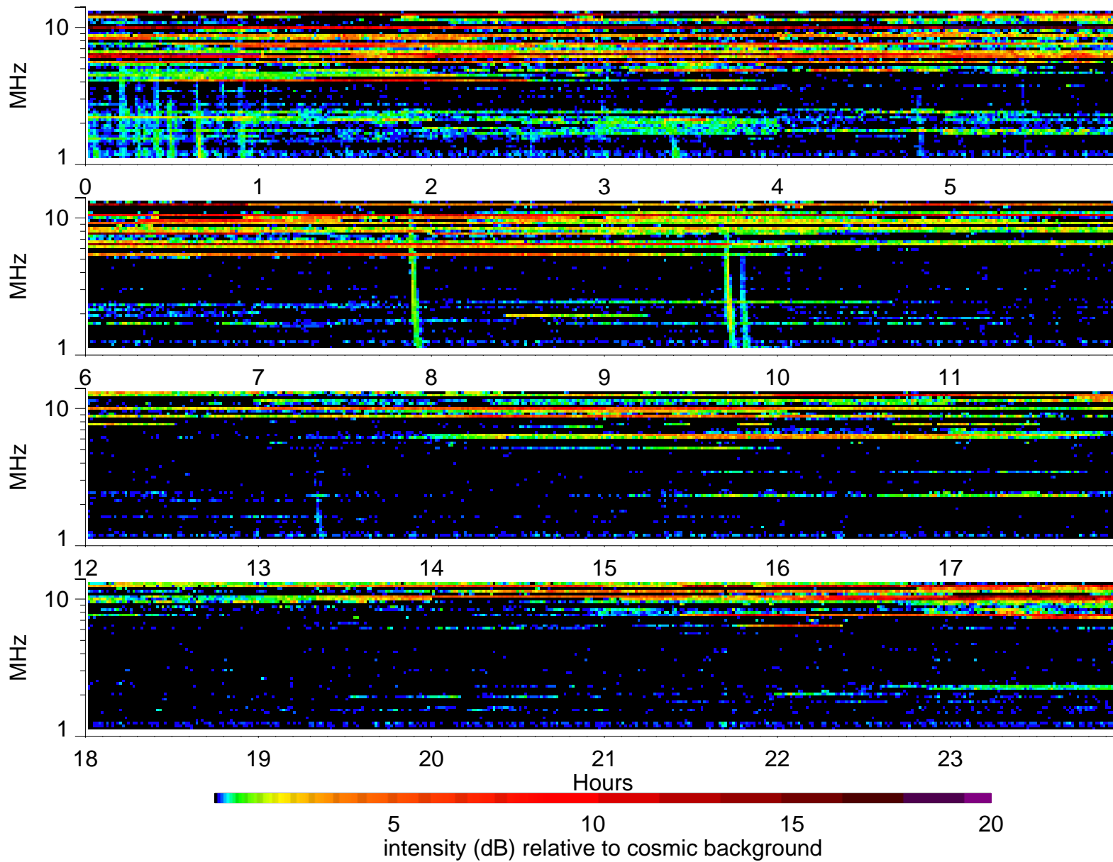
Wind Waves RAD2 receiver: 1999/4/25
