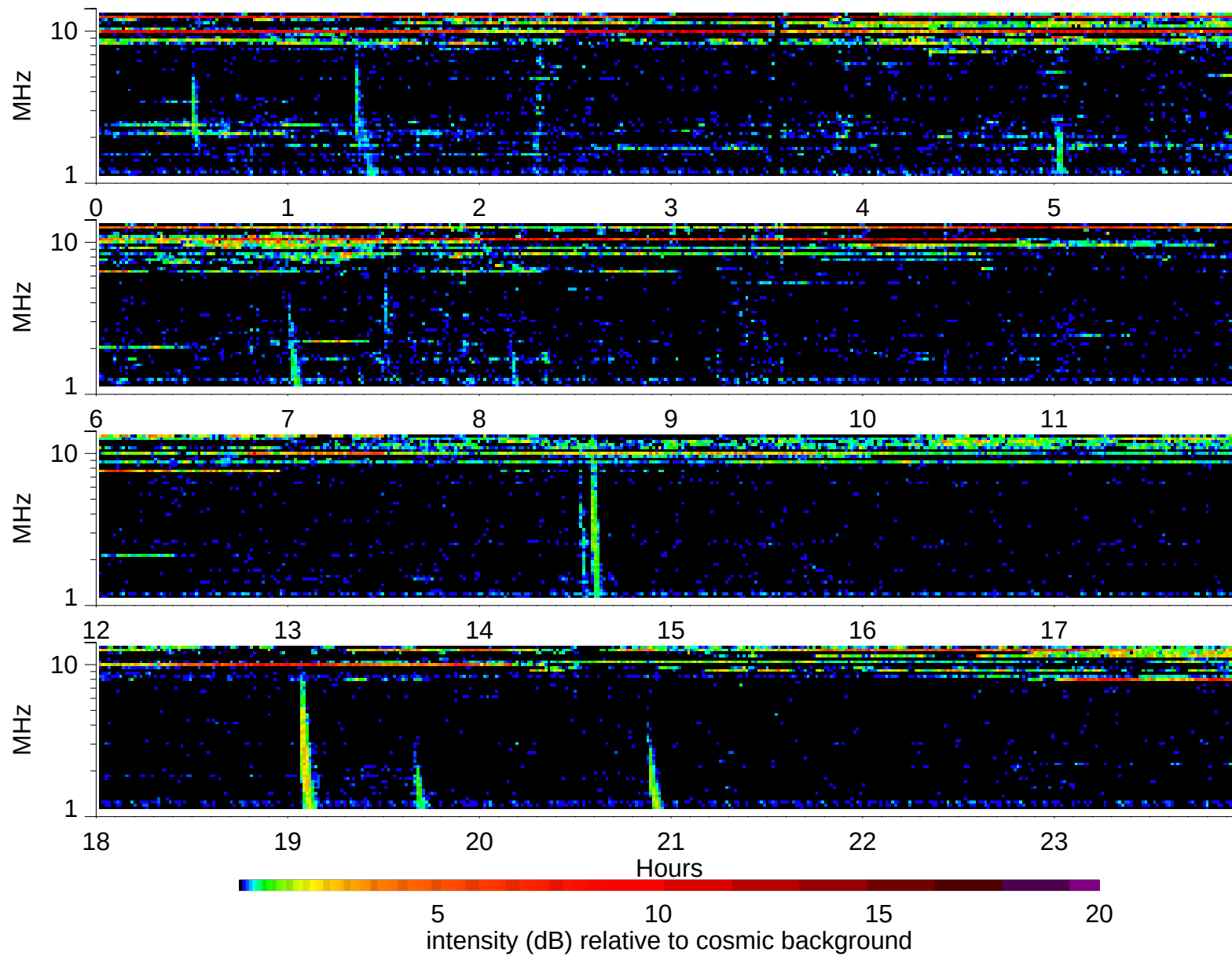
Wind Waves RAD2 receiver: 1999/4/27
