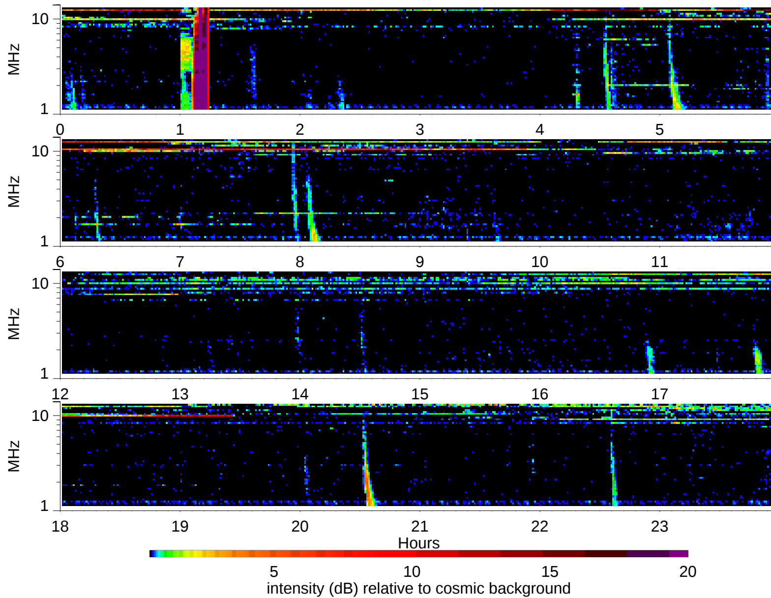
Wind Waves RAD2 receiver: 1999/4/28
