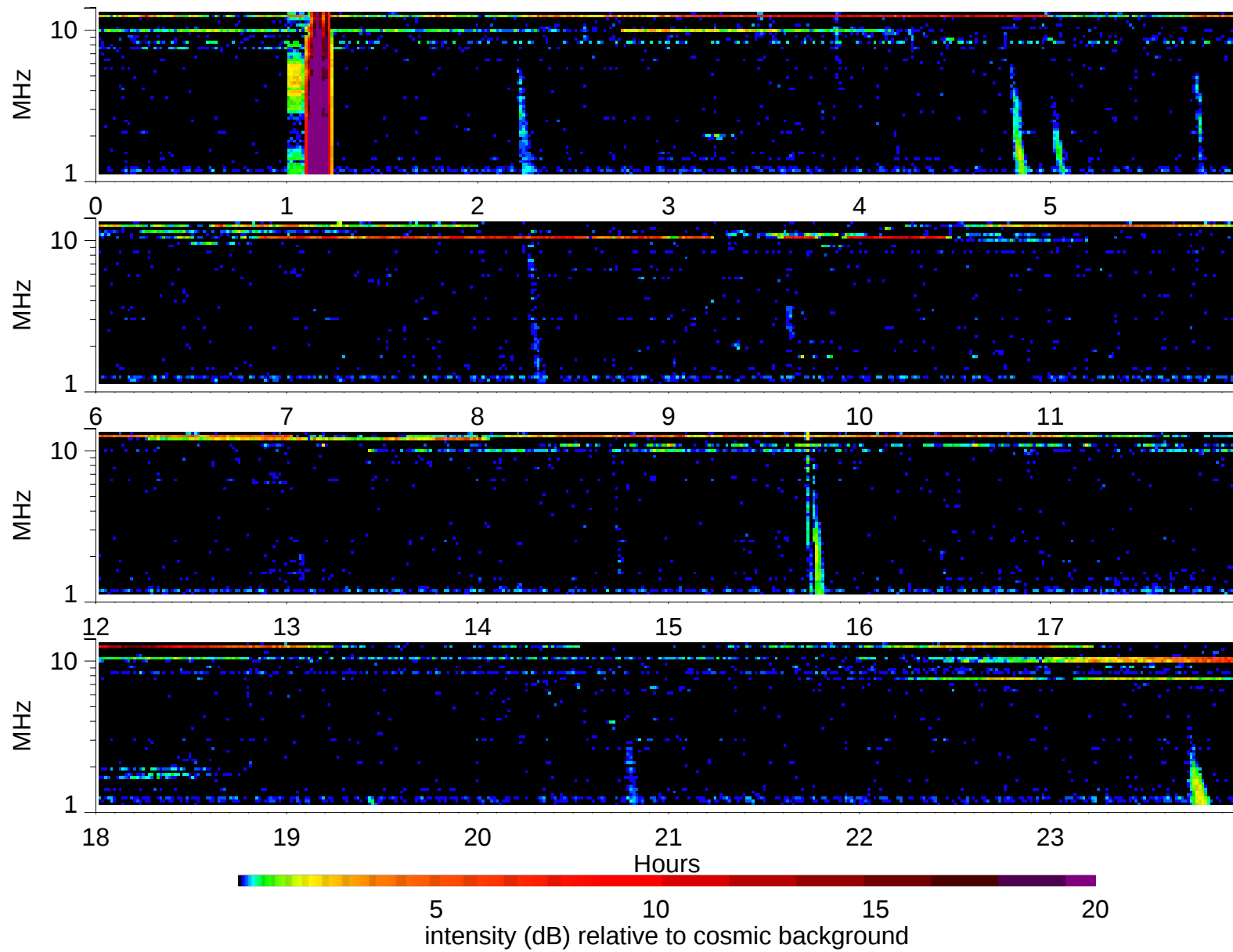
Wind Waves RAD2 receiver: 1999/4/30
