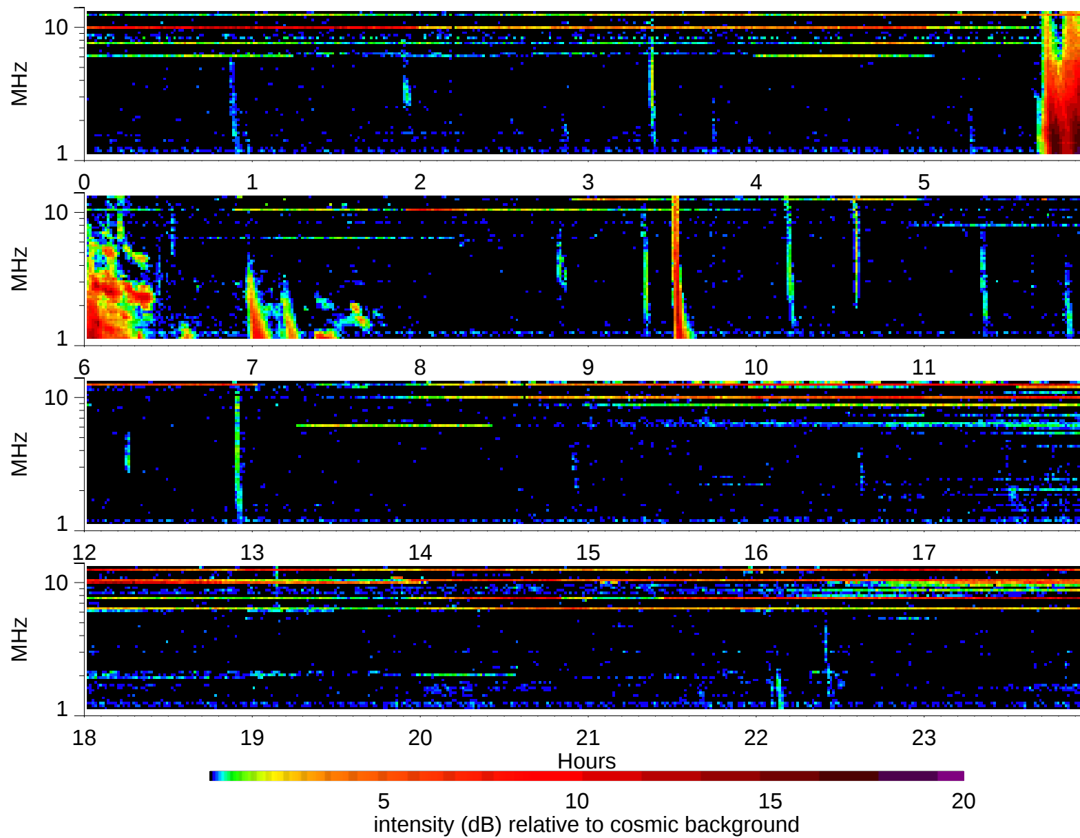
Wind Waves RAD2 receiver: 1999/5/3
