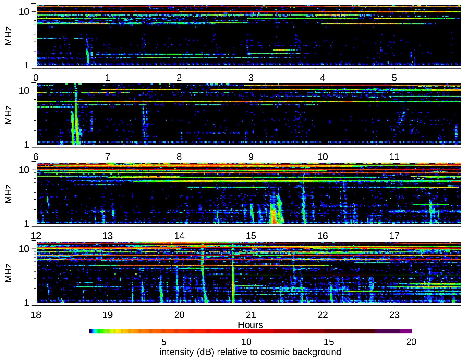
Wind Waves RAD2 receiver: 1999/5/5
