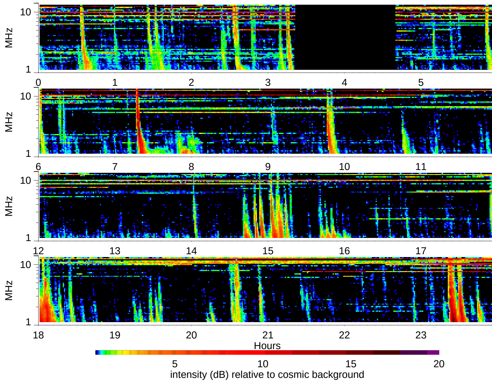
Wind Waves RAD2 receiver: 1999/5/9
