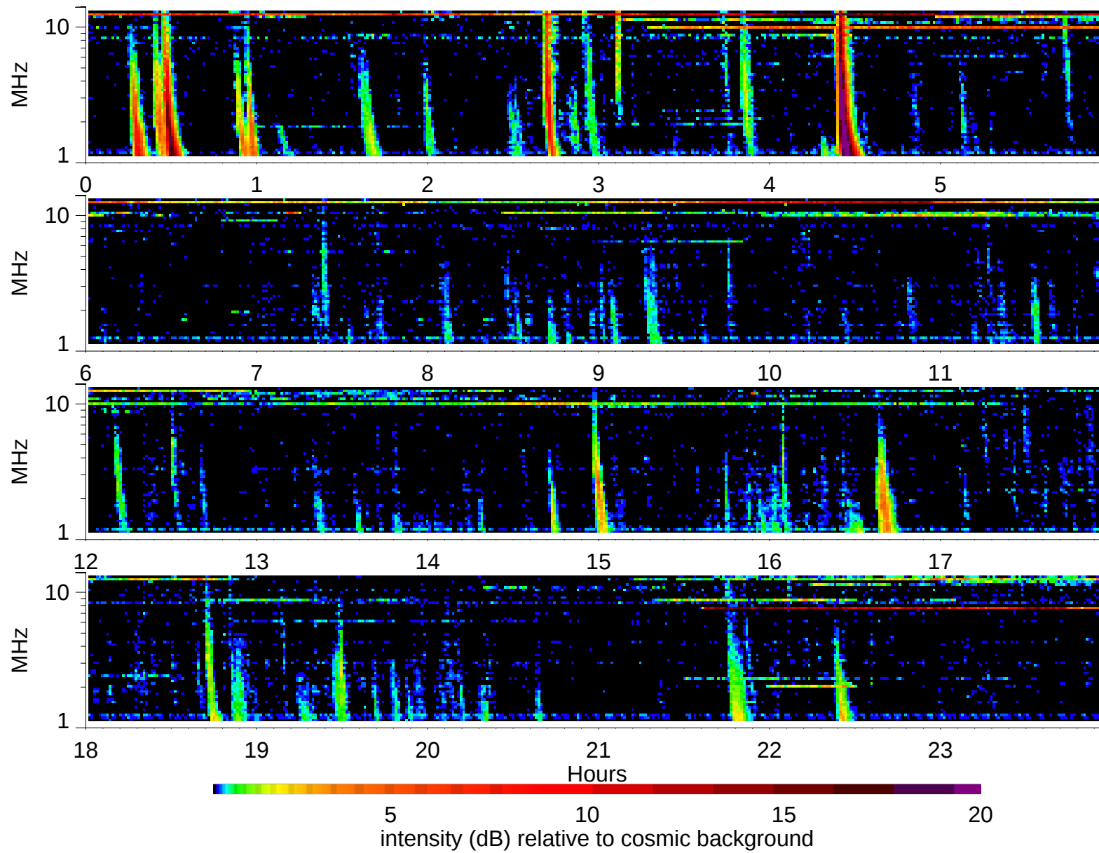
Wind Waves RAD2 receiver: 1999/5/11
