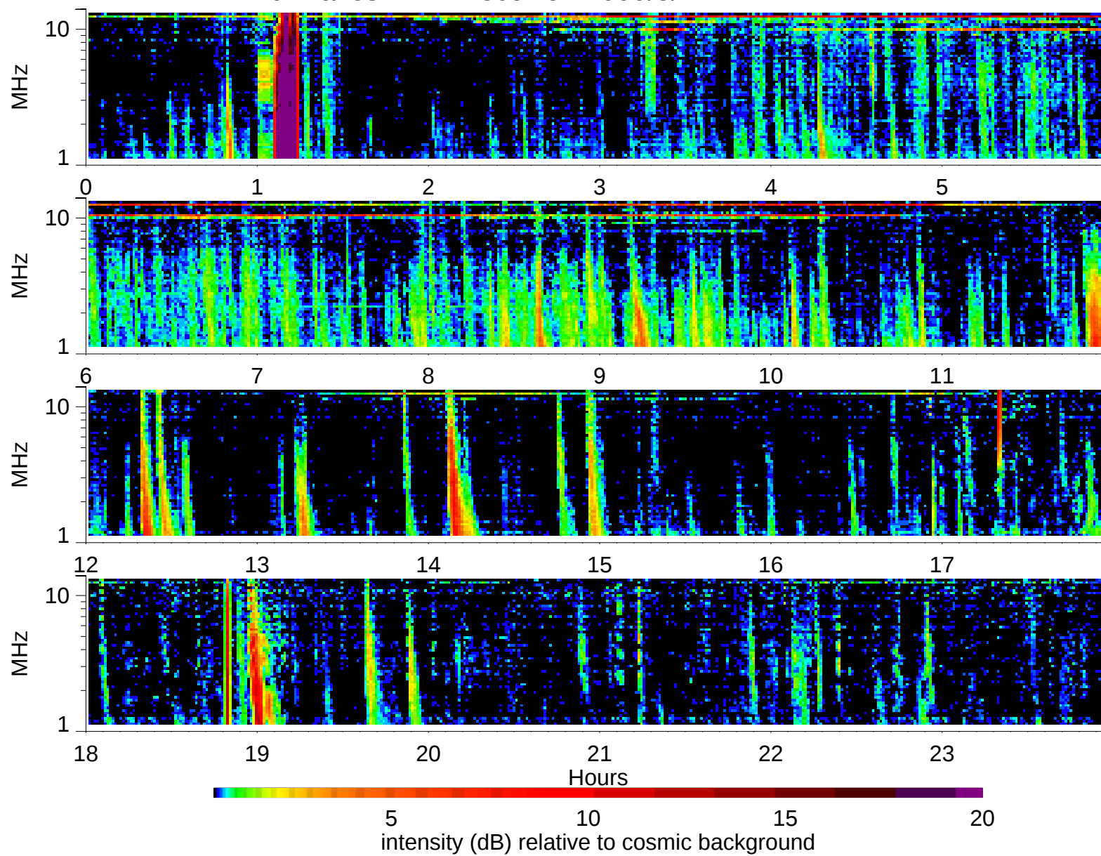
Wind Waves RAD2 receiver: 1999/5/14
