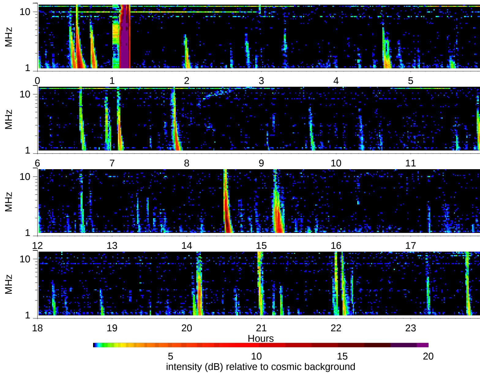
Wind Waves RAD2 receiver: 1999/5/22
