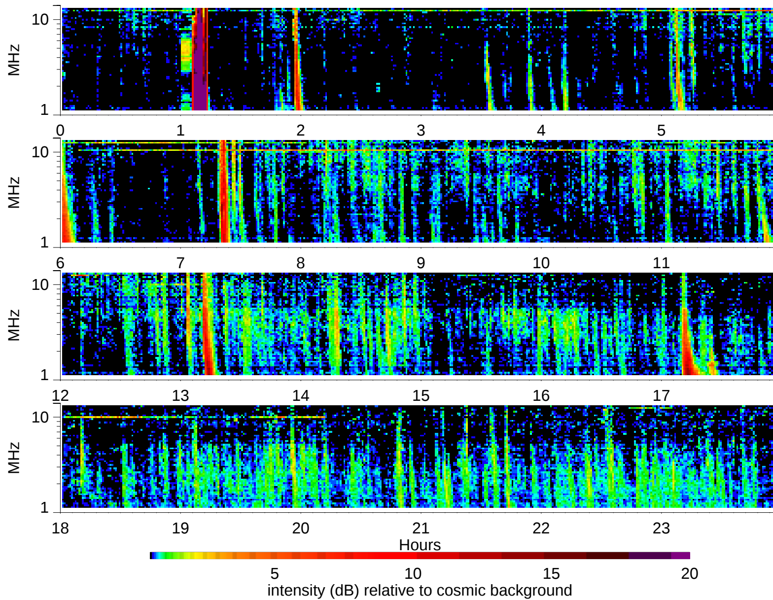
Wind Waves RAD2 receiver: 1999/5/24
