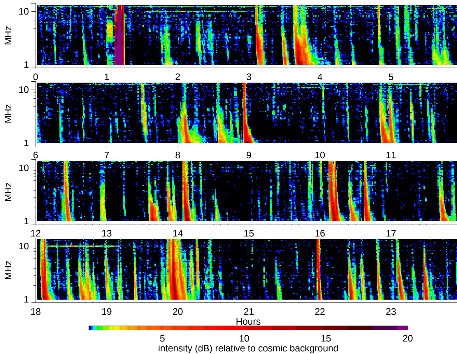
Wind Waves RAD2 receiver: 1999/5/26
