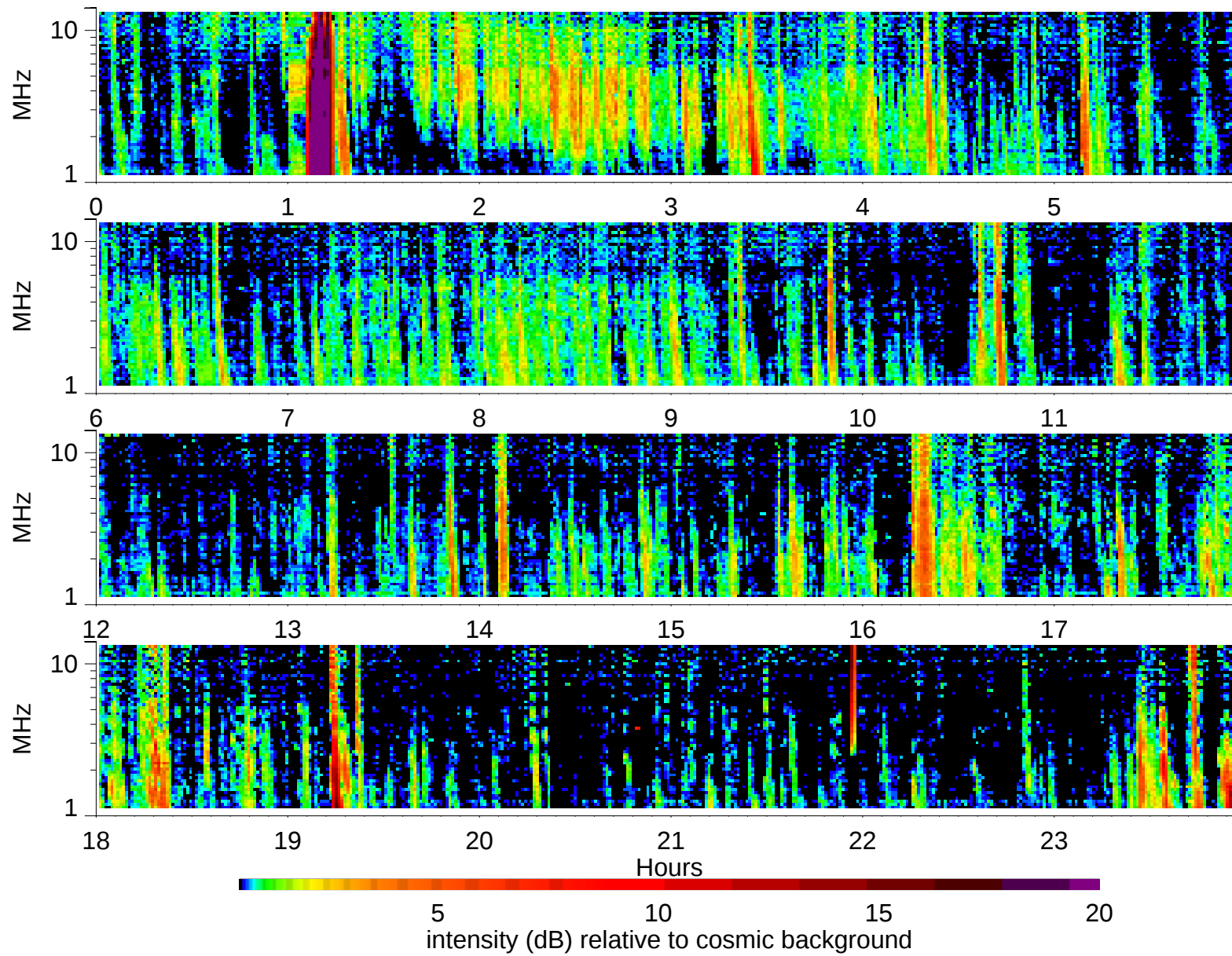
Wind Waves RAD2 receiver: 1999/5/30
