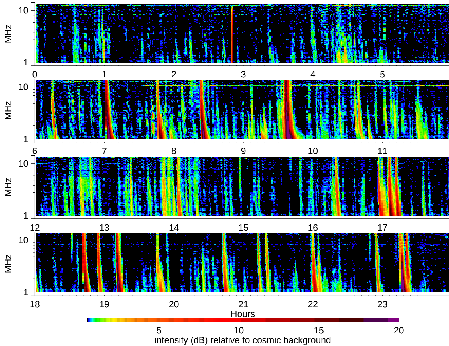
Wind Waves RAD2 receiver: 1999/5/31
