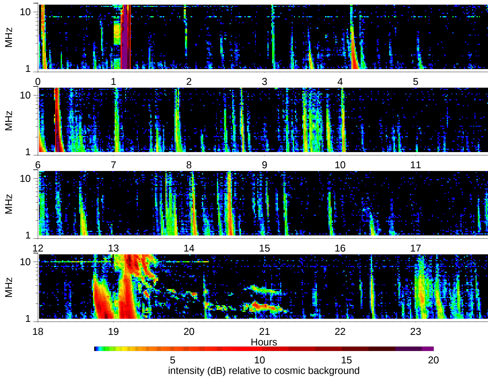
Wind Waves RAD2 receiver: 1999/6/1
