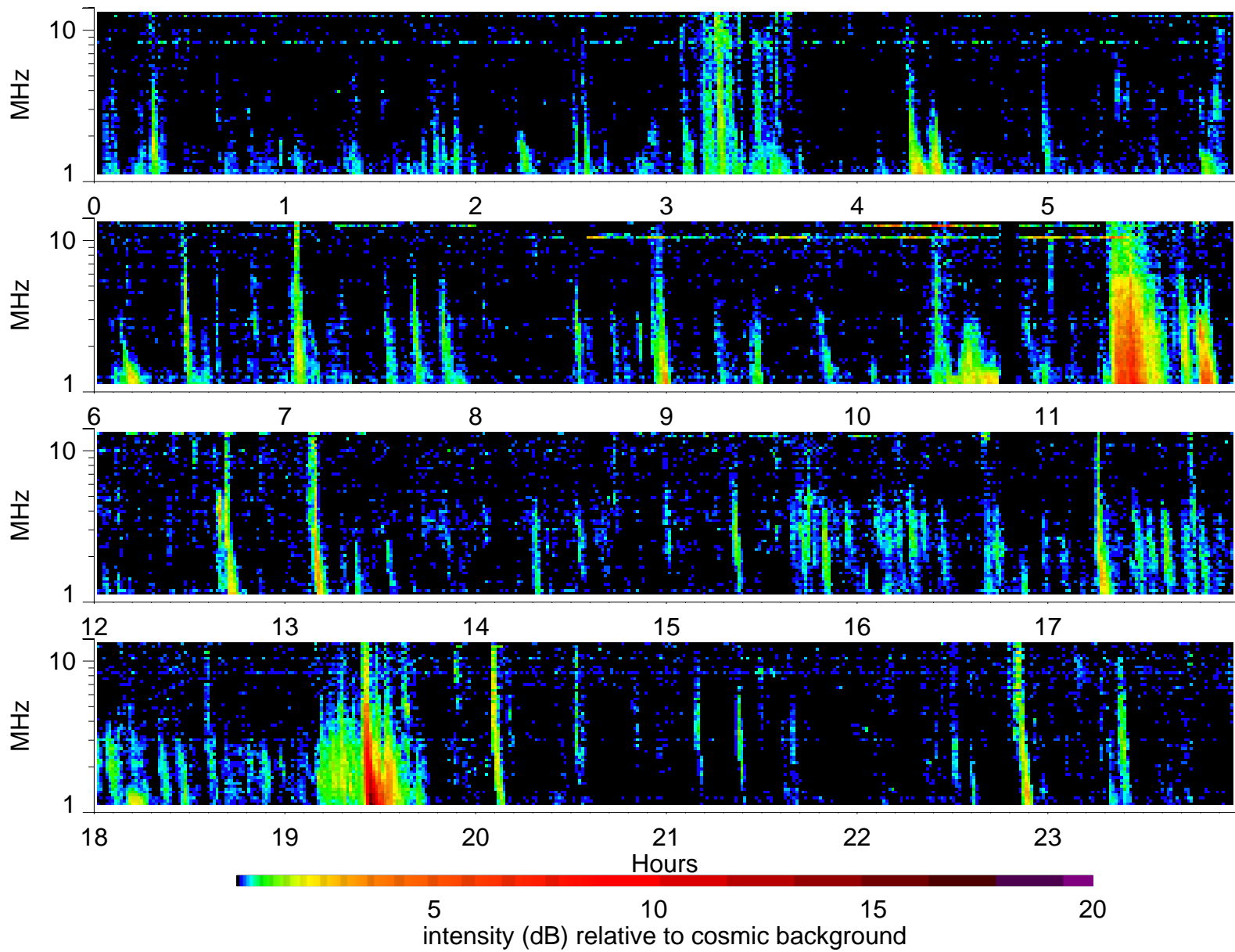
Wind Waves RAD2 receiver: 1999/6/2
