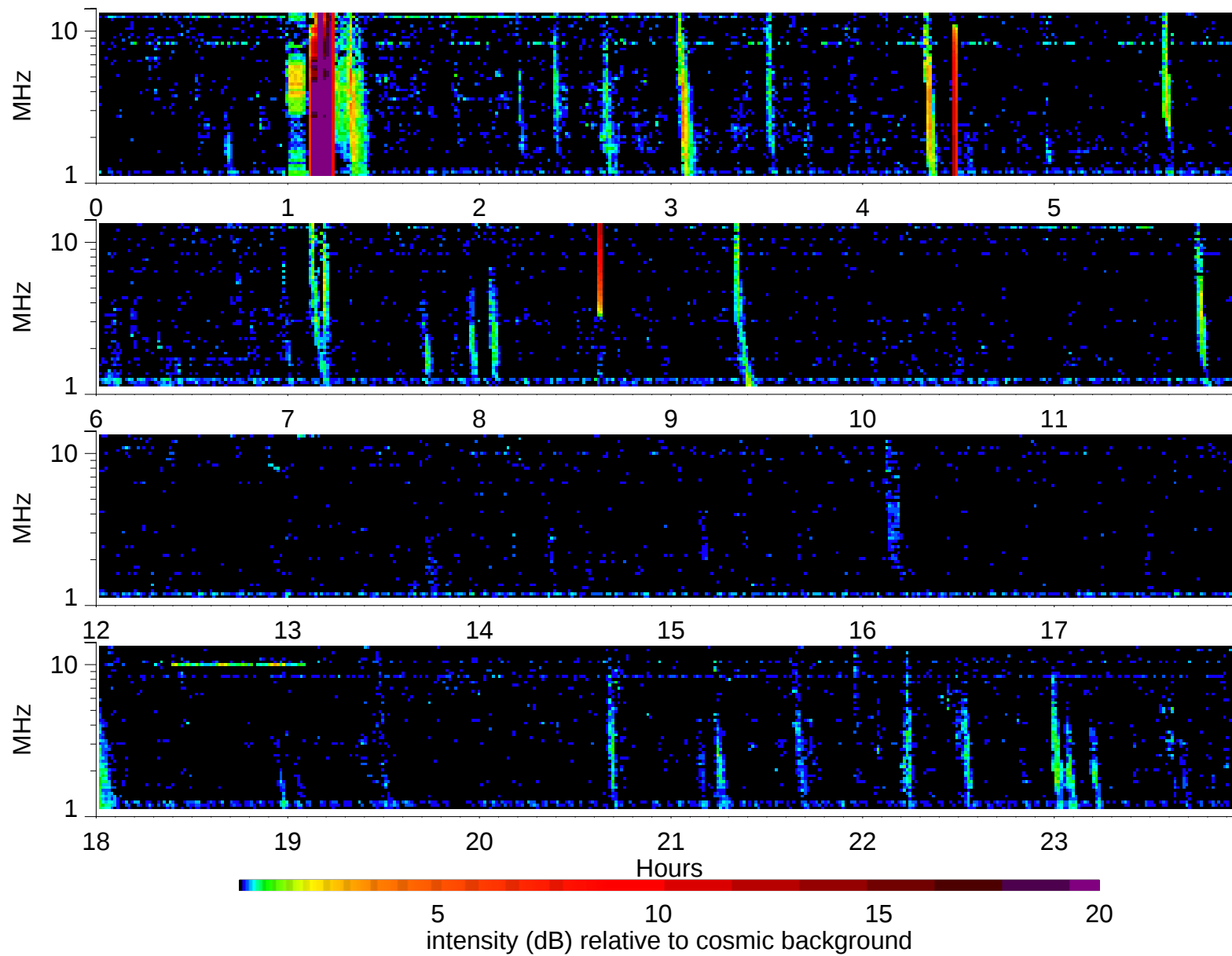
Wind Waves RAD2 receiver: 1999/6/5
