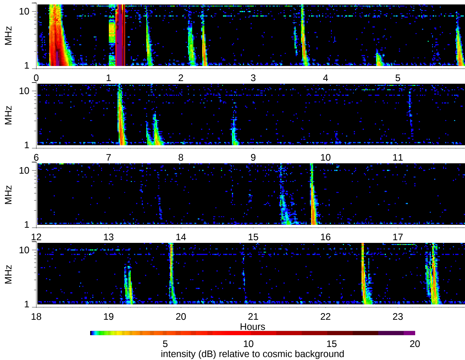
Wind Waves RAD2 receiver: 1999/6/9
