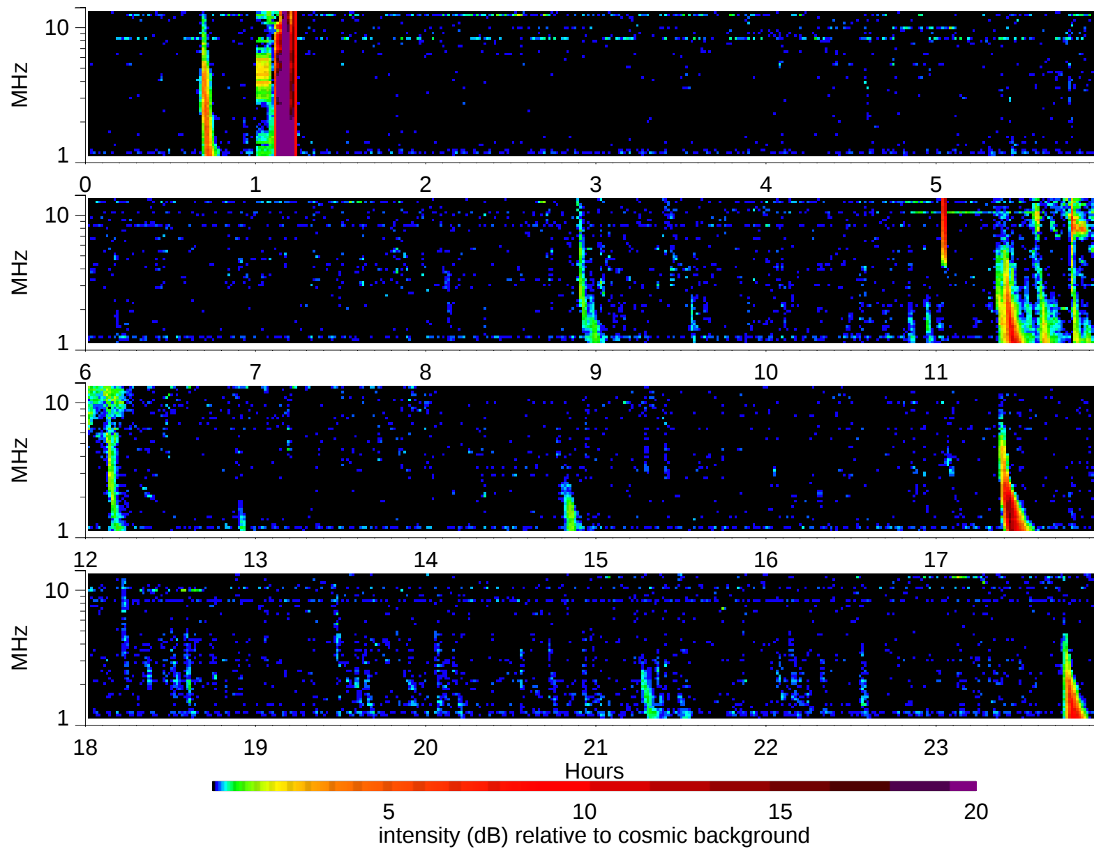
Wind Waves RAD2 receiver: 1999/6/11
