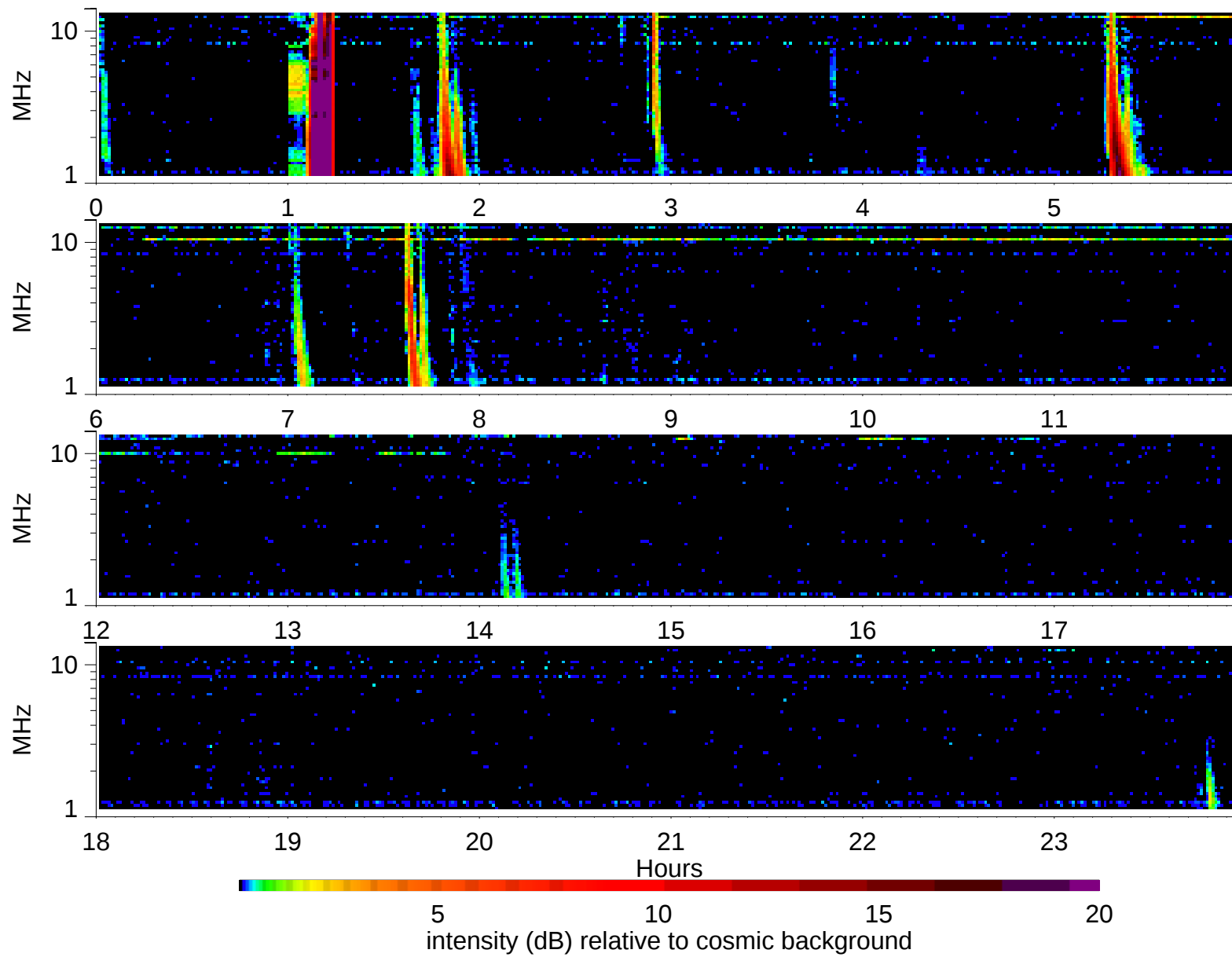
Wind Waves RAD2 receiver: 1999/6/13
