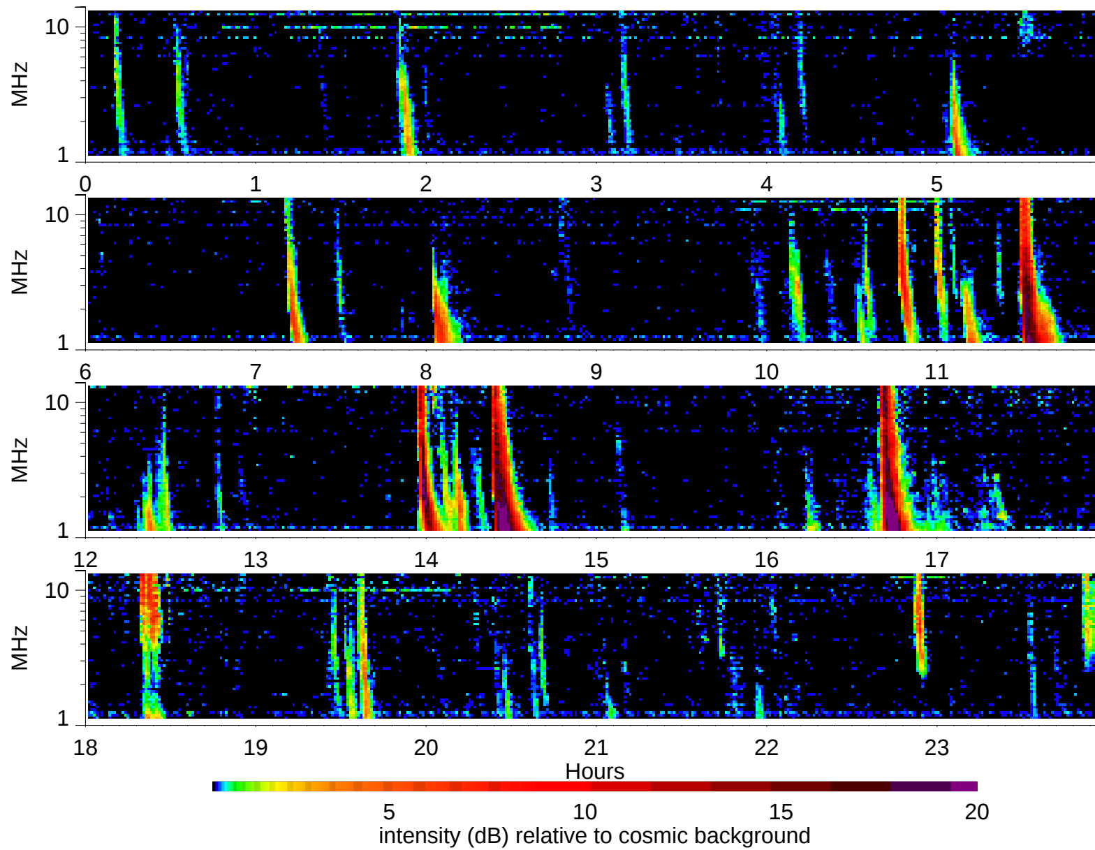
Wind Waves RAD2 receiver: 1999/6/18
