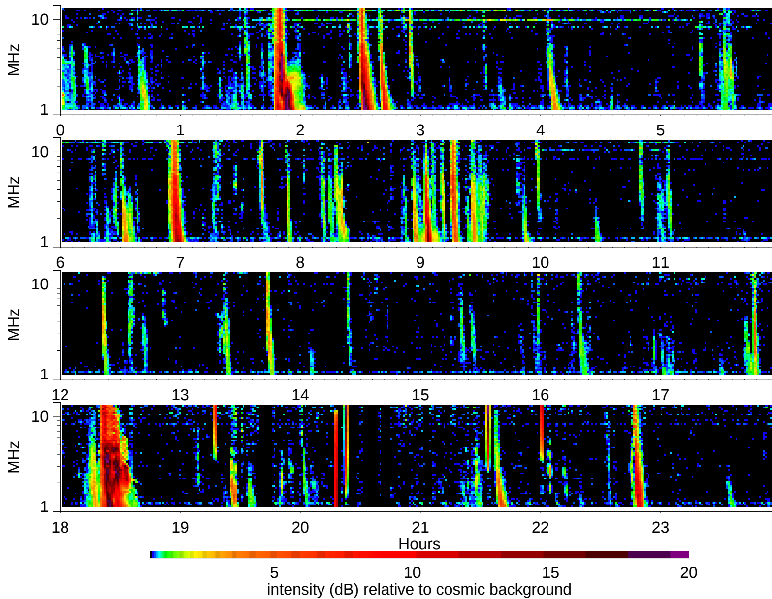
Wind Waves RAD2 receiver: 1999/6/22
