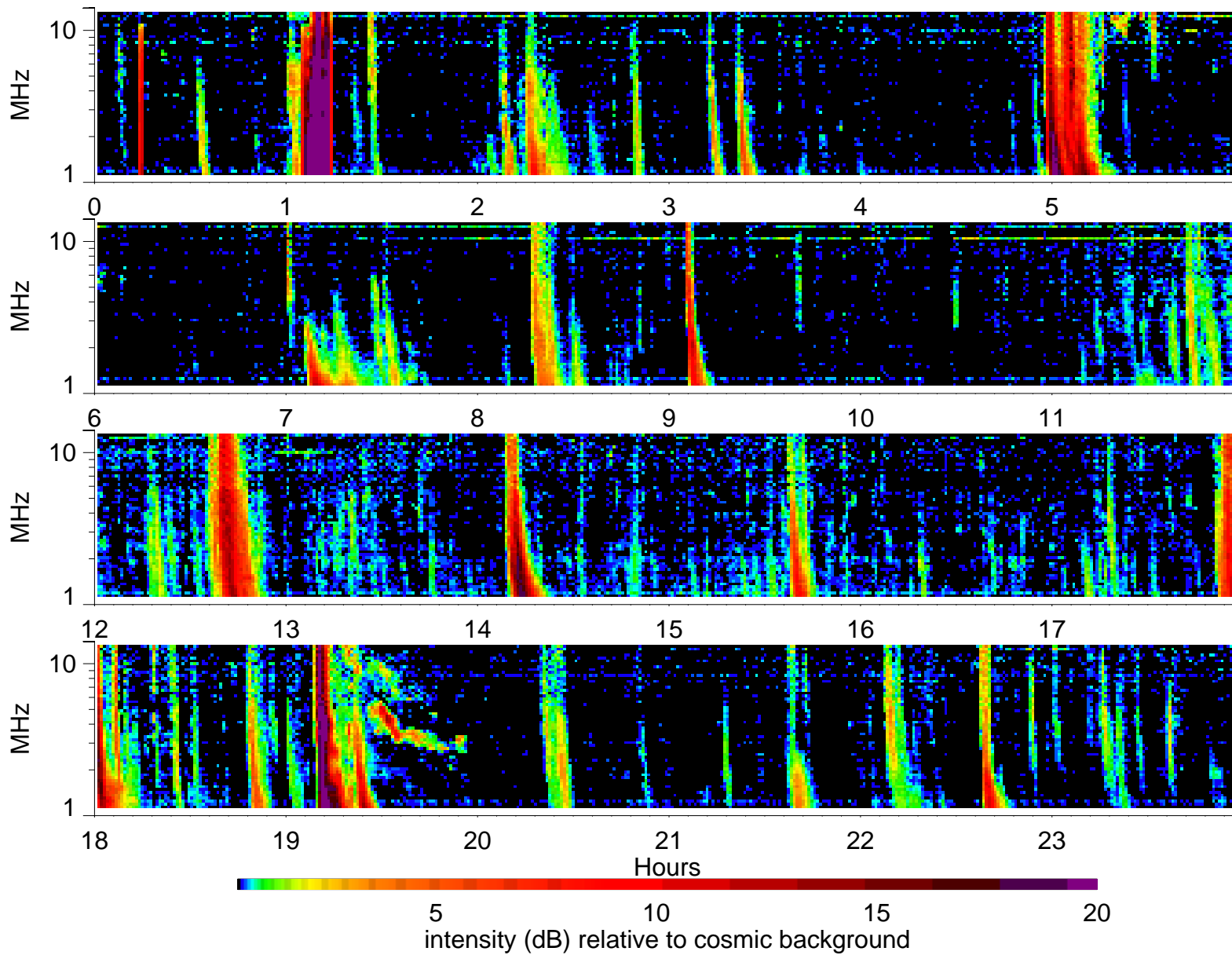
Wind Waves RAD2 receiver: 1999/6/29
