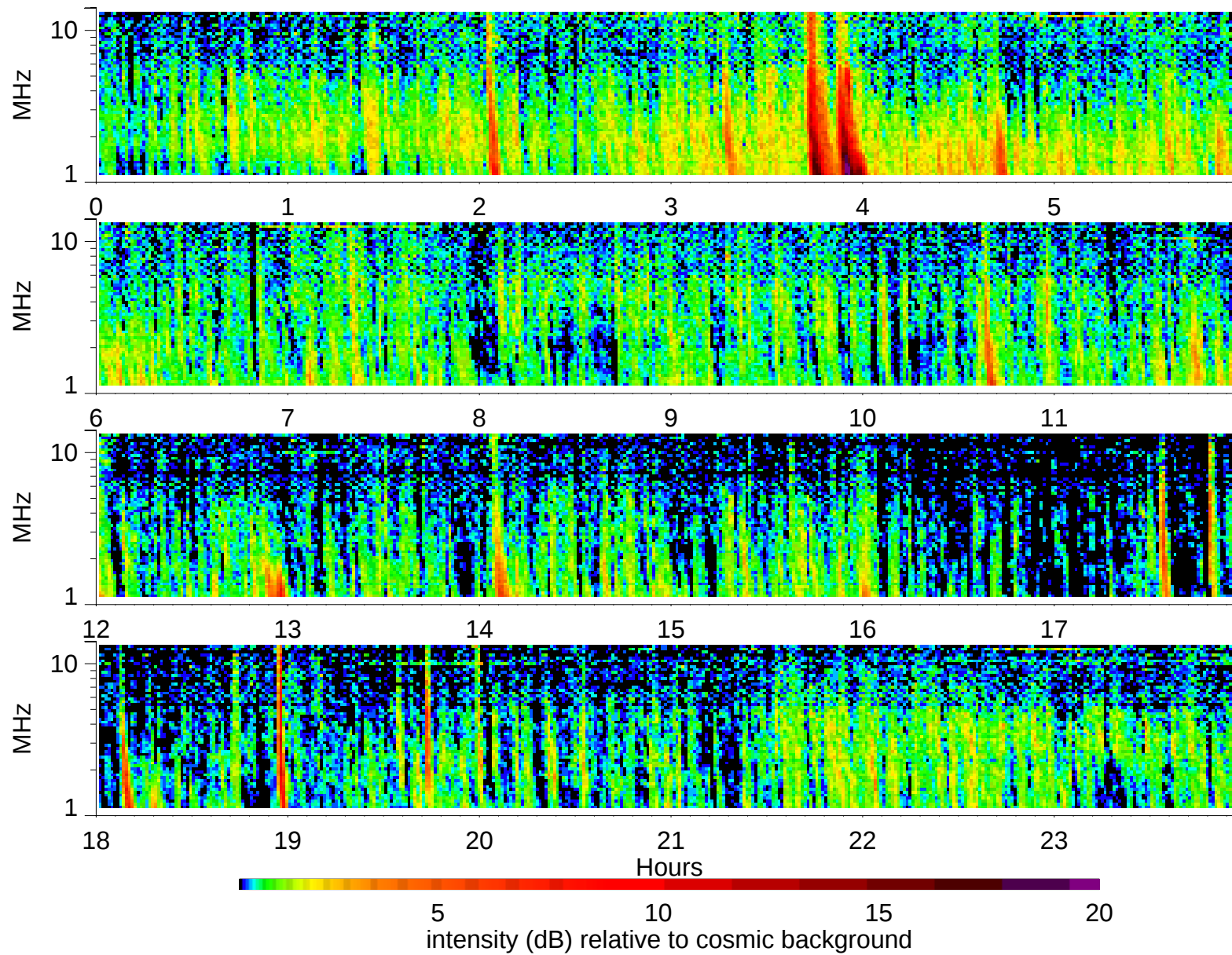
Wind Waves RAD2 receiver: 1999/7/2
