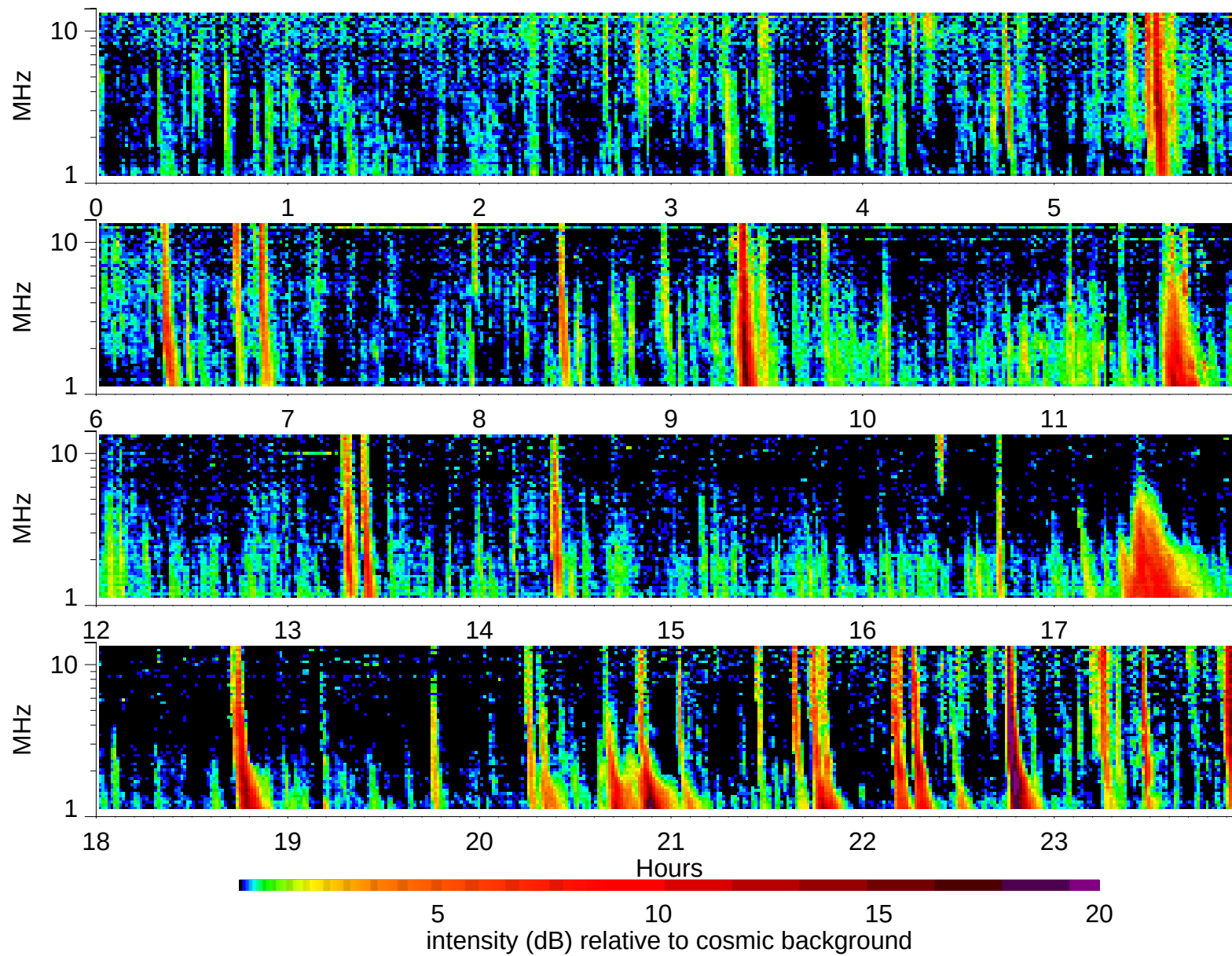
Wind Waves RAD2 receiver: 1999/7/4
