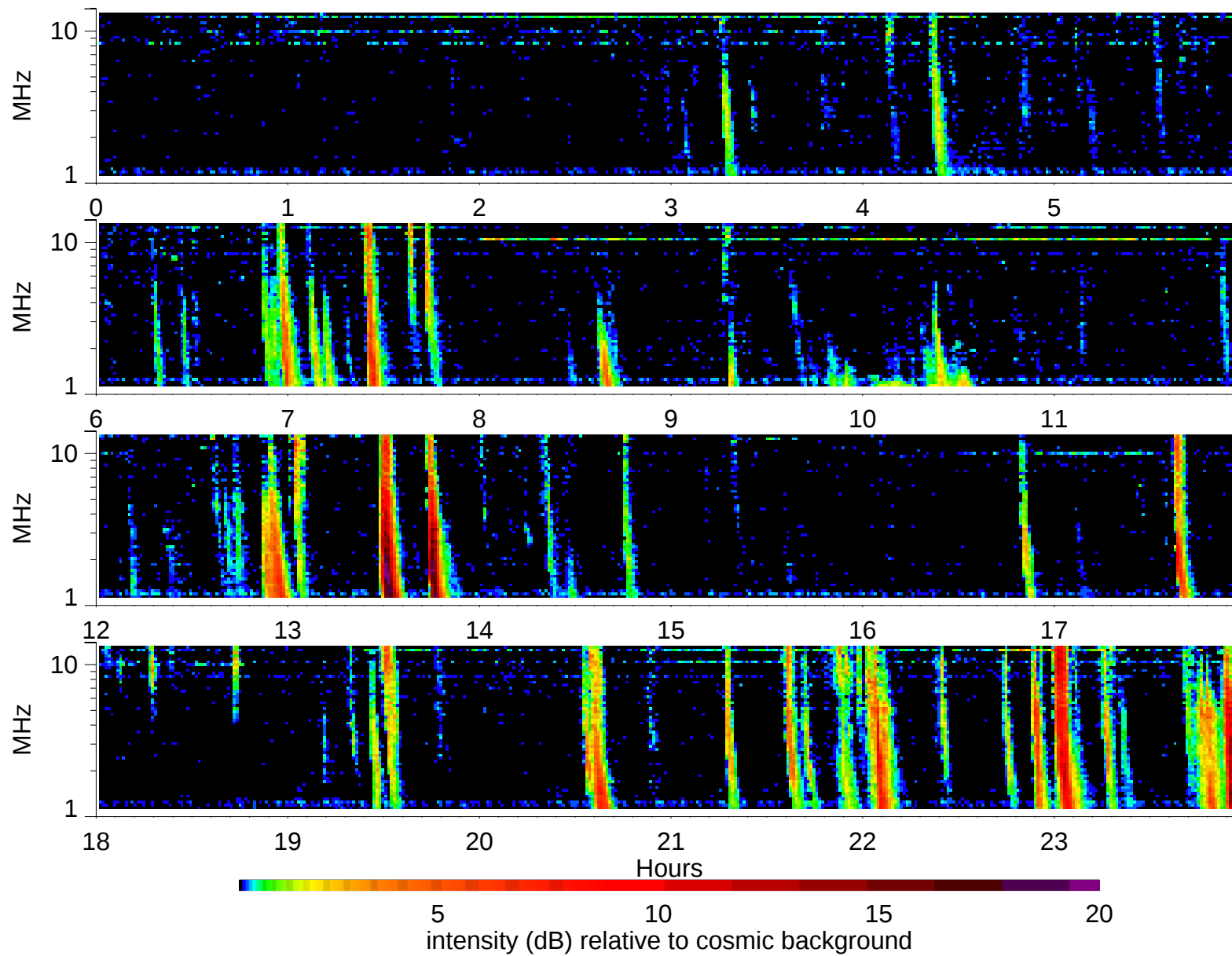
Wind Waves RAD2 receiver: 1999/7/8
