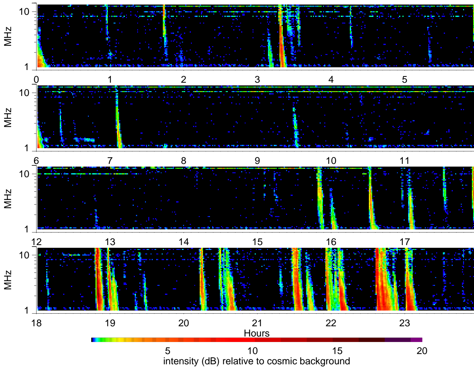
Wind Waves RAD2 receiver: 1999/7/10
