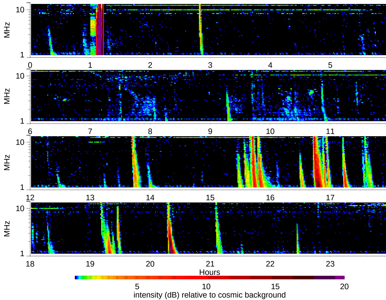
Wind Waves RAD2 receiver: 1999/7/17
