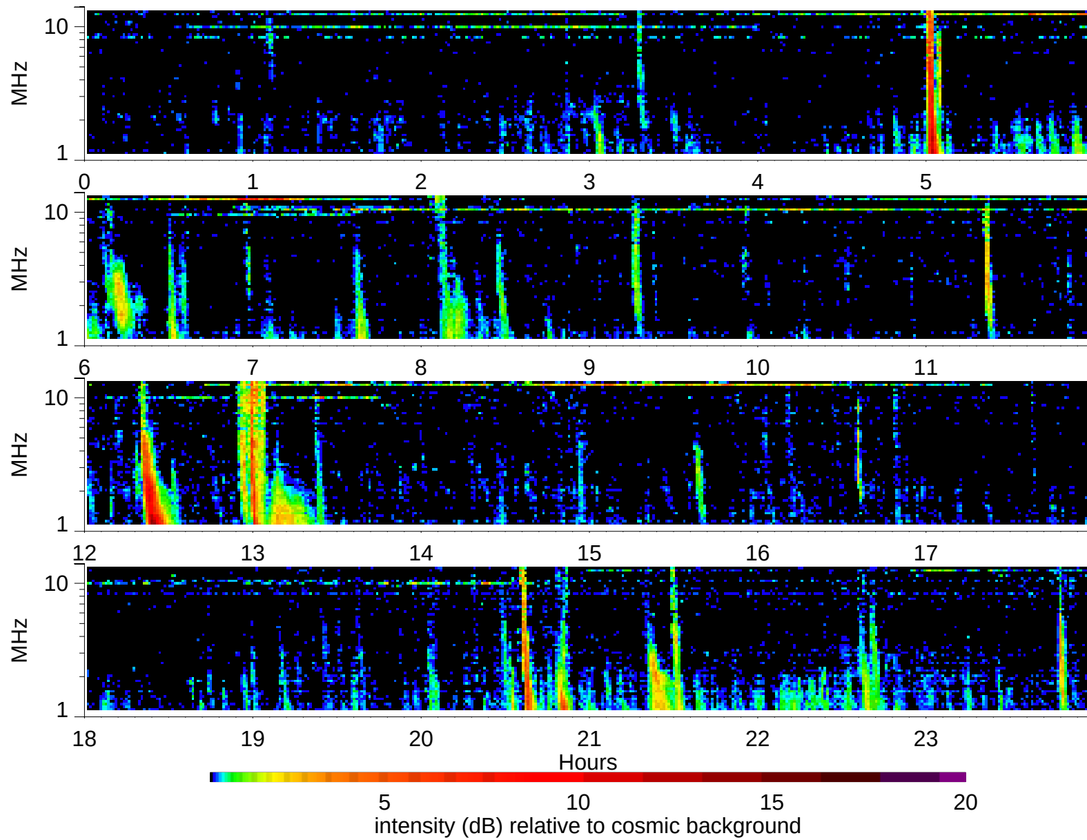
Wind Waves RAD2 receiver: 1999/7/24
