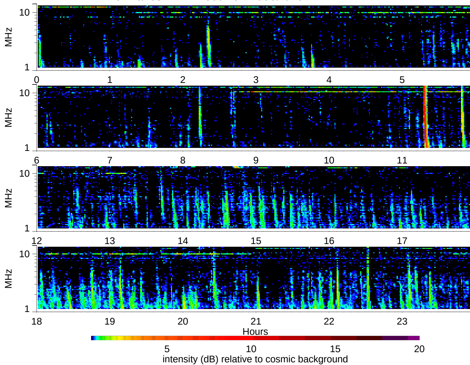
Wind Waves RAD2 receiver: 1999/7/26
