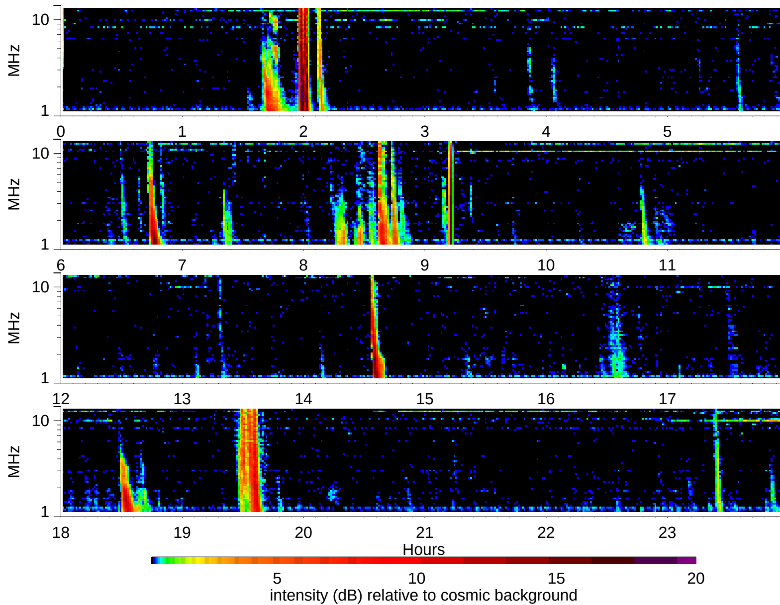
Wind Waves RAD2 receiver: 1999/7/28
