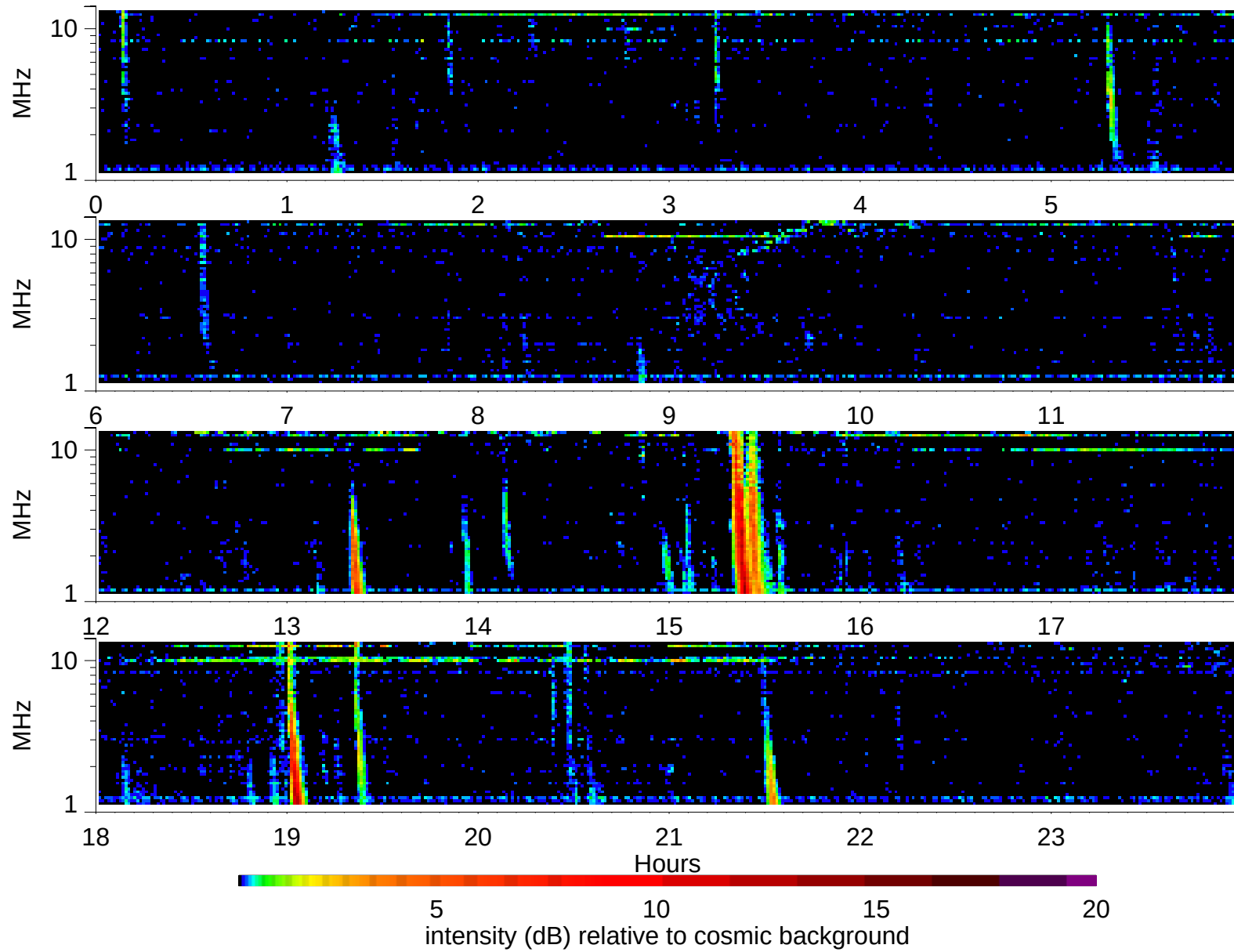
Wind Waves RAD2 receiver: 1999/7/30
